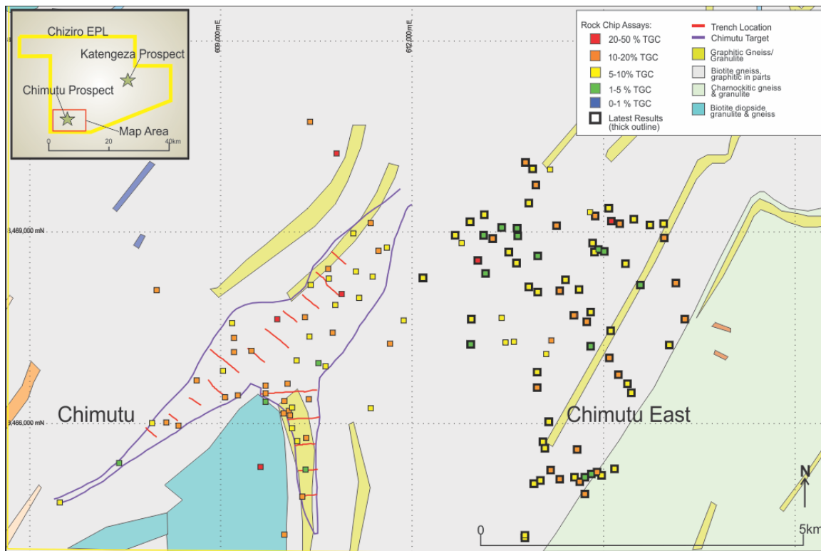
Figure 2: Chimutu and Chimutu East Prospect rock chip results. Assays received during the March Quarter are highlighted with a thick black outline.
