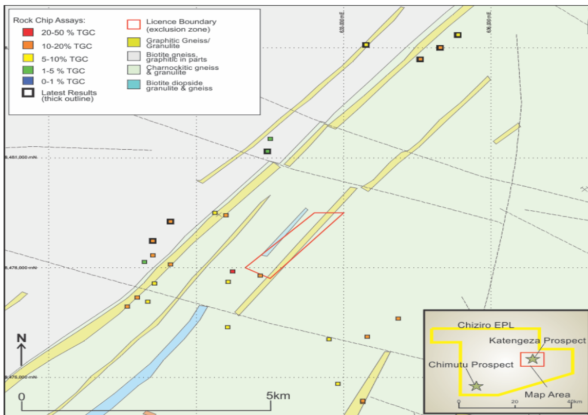
Figure 3: Katengeza Prospect rock chip results. Assays received during the March Quarter are highlighted with a thick black outline.
