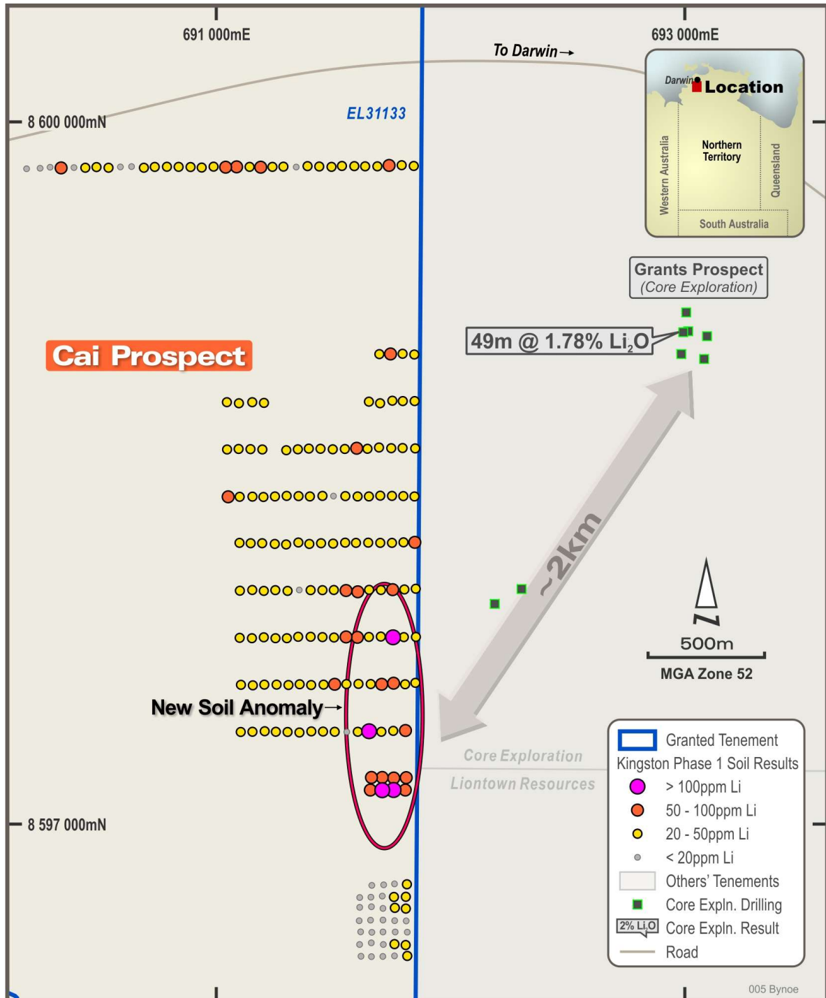
Figure 2: EL31133 Cai Prospect lithium in soil anomaly (CXO drillhole locations extracted from its ASX announcement dated 20 th October 2016)
