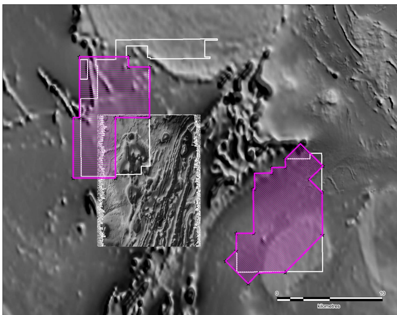
Figure 1. Planned high resolution aeromagnetic survey (magenta) over Celsius tenements (white) and public domain aeromagnetic data available from the Geological Survey of Western Australia.
