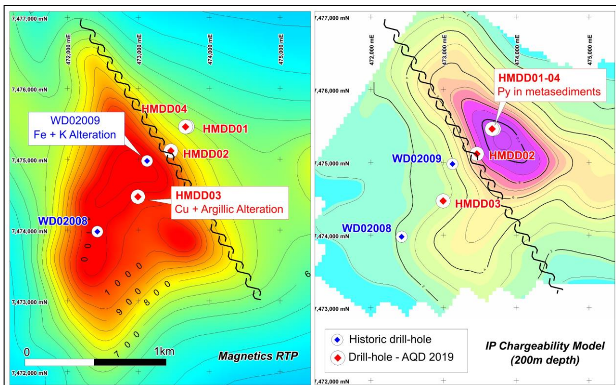
Figure 1: Hamilton Project showing recent drill-hole locations
