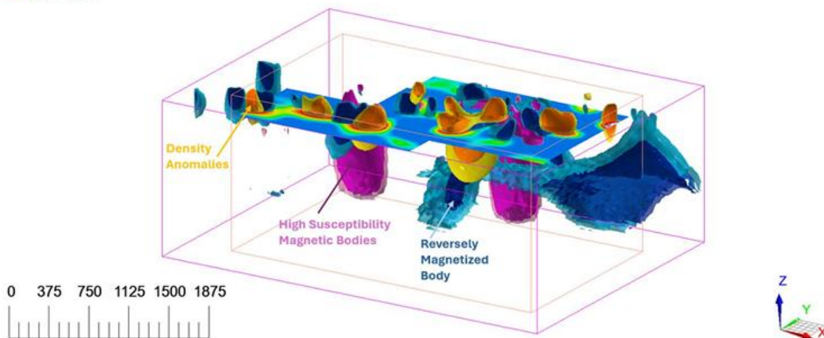
Figure 16. Dumunzi magnetic and density 3D inversion models showing the relationship between different magnetic units within a structurally-complex zone.
