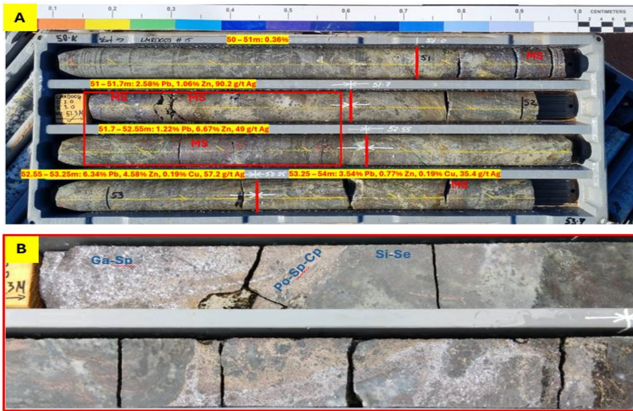
Figure 14. A. Diamond Drill core of LMRD004 50.4 – 53.7m, showing zones of massive sulphide within silica-sericite-altered and folded Lander Rock Formation. B. Close-up of cut core from red box in A showing massive pyrrhotite-sphalerite-chalcopyrite cut by galena-sphalerite within strong silica-sericite-altered Lander Rock Formation.
