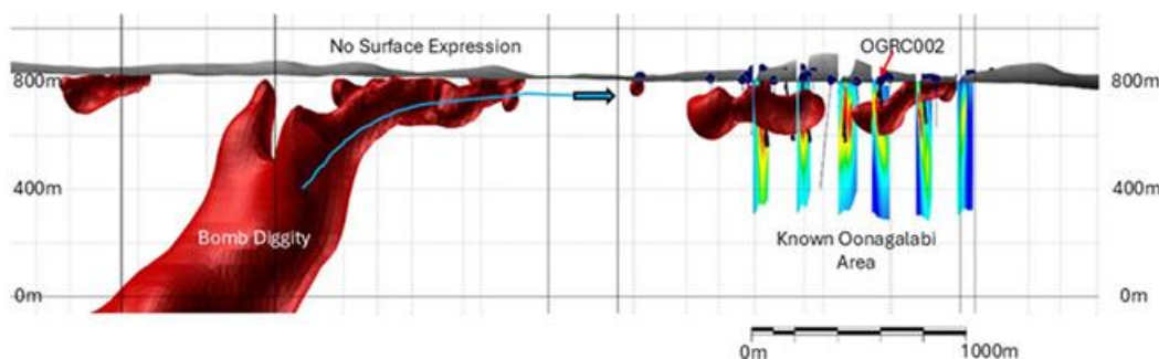
Figure 8. Long section between Bomb Diggity and Oonagalabi (looking southeast) showing the Bomb Diggity magnetic anomaly (red polygons, >0.022 mesh) and interpreted hydrothermal fluid outflow into the Oonagalabi system. OGRC002 intersected 15m @ 0.45 g/t Ag, 0.17% Bi within semi-massive magnetite alteration that appears to overprint earlier carbonate-replacement Cu-Zn mineralisation.
