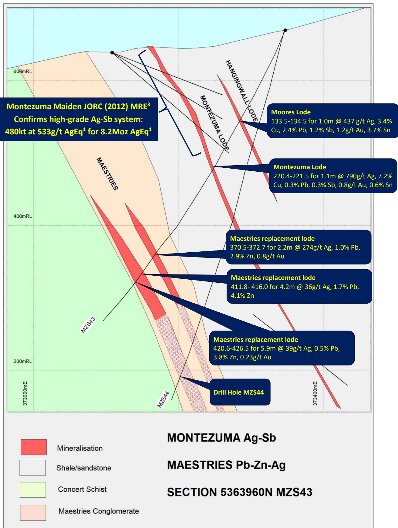
Figure 1 Schematic cross section 5363960N, MZS43 with mineralised intercepts.
