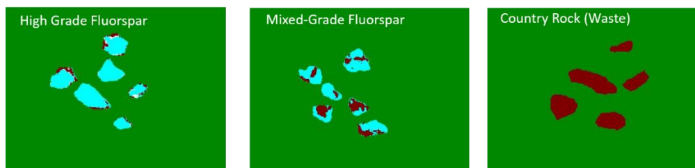
Figure 10: Laser ore-sorting technology by TOMRA applied to Quinn Project metallurgical samples. This clearly differentiates ore types and provides low-cost path to upgrade of mineral products with coarse crush only. Samples approximately 10-15mm
