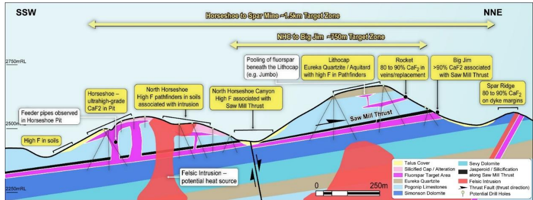
Figure 6: Schematic cross-section from Horseshoe to Big Jim/Spar, with preliminary drill designs
