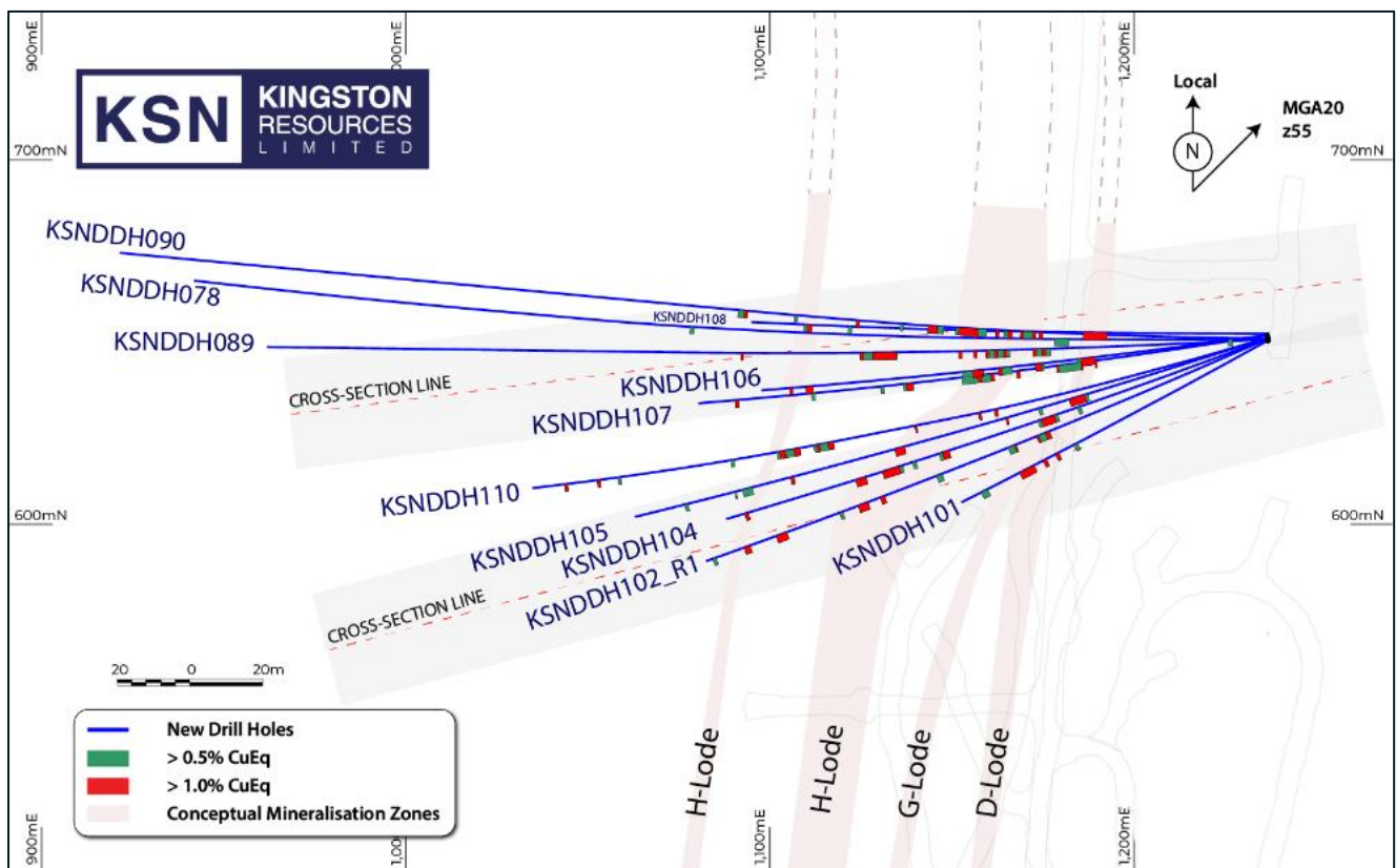
Figure 1: Plan view of the recent northern extension drilling targeting D, G and H Lodes
