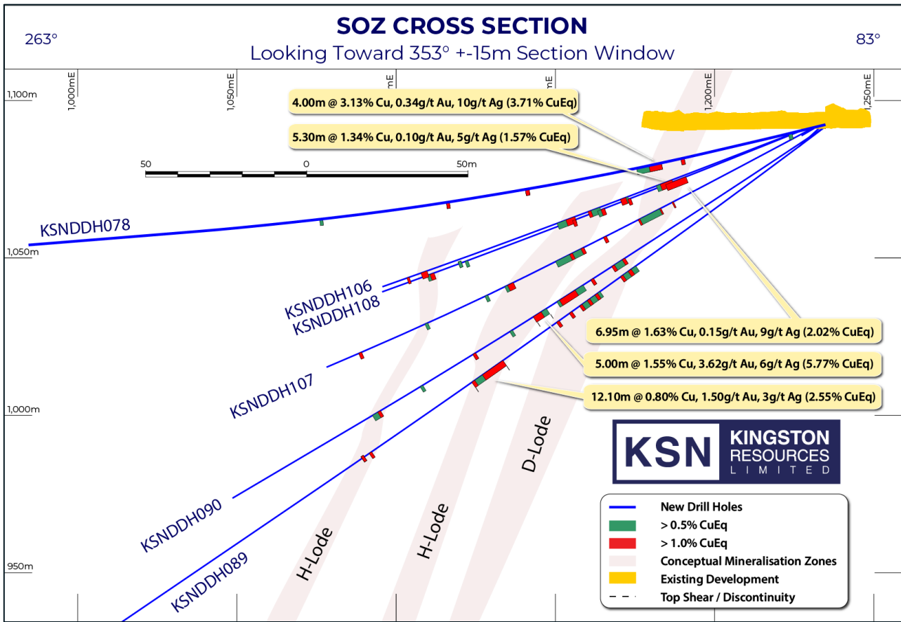
Figure 4: Oblique cross section of the northern group of drill holes.
