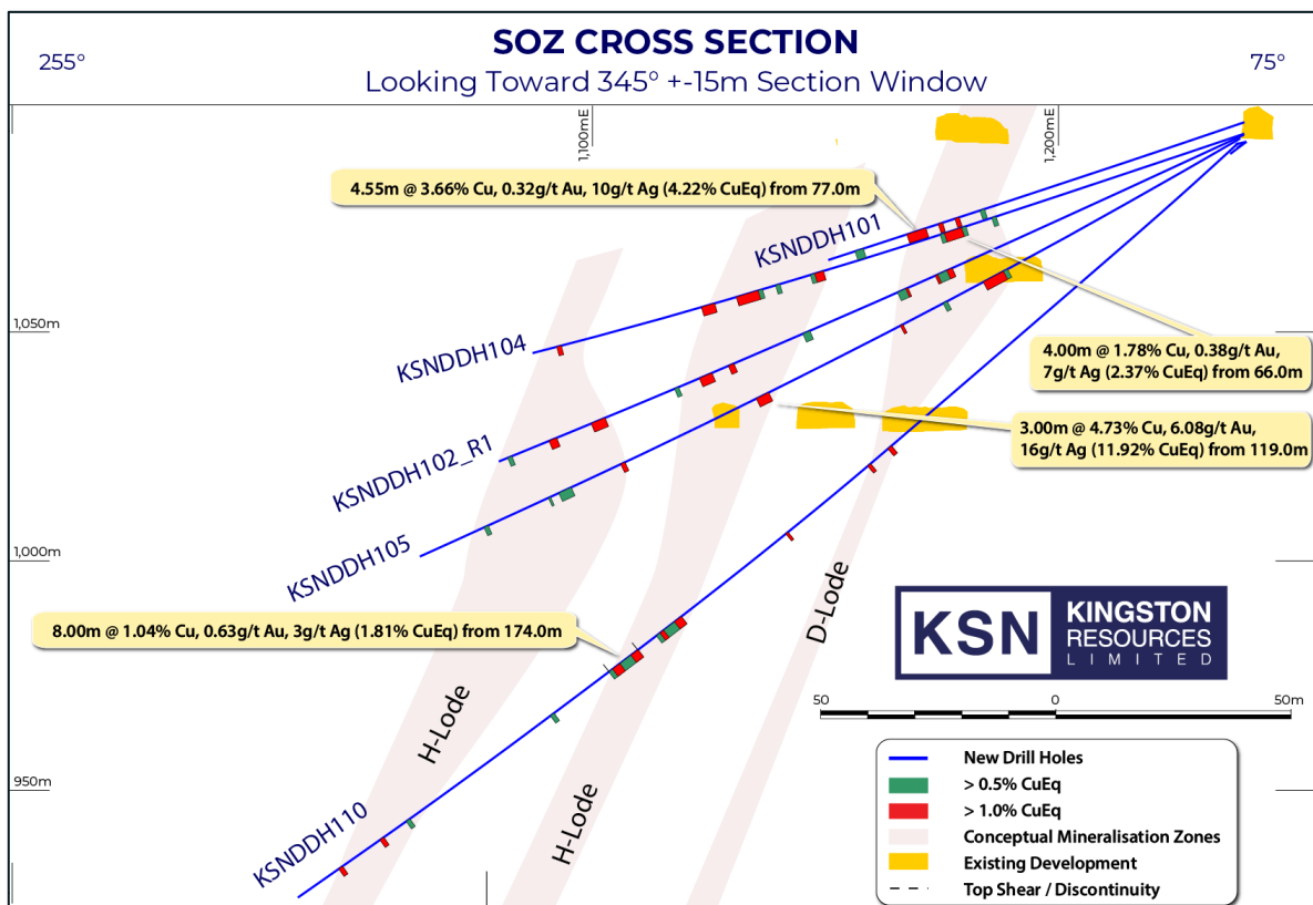
Figure 3: Oblique cross section looking at the southern group of drill holes.
