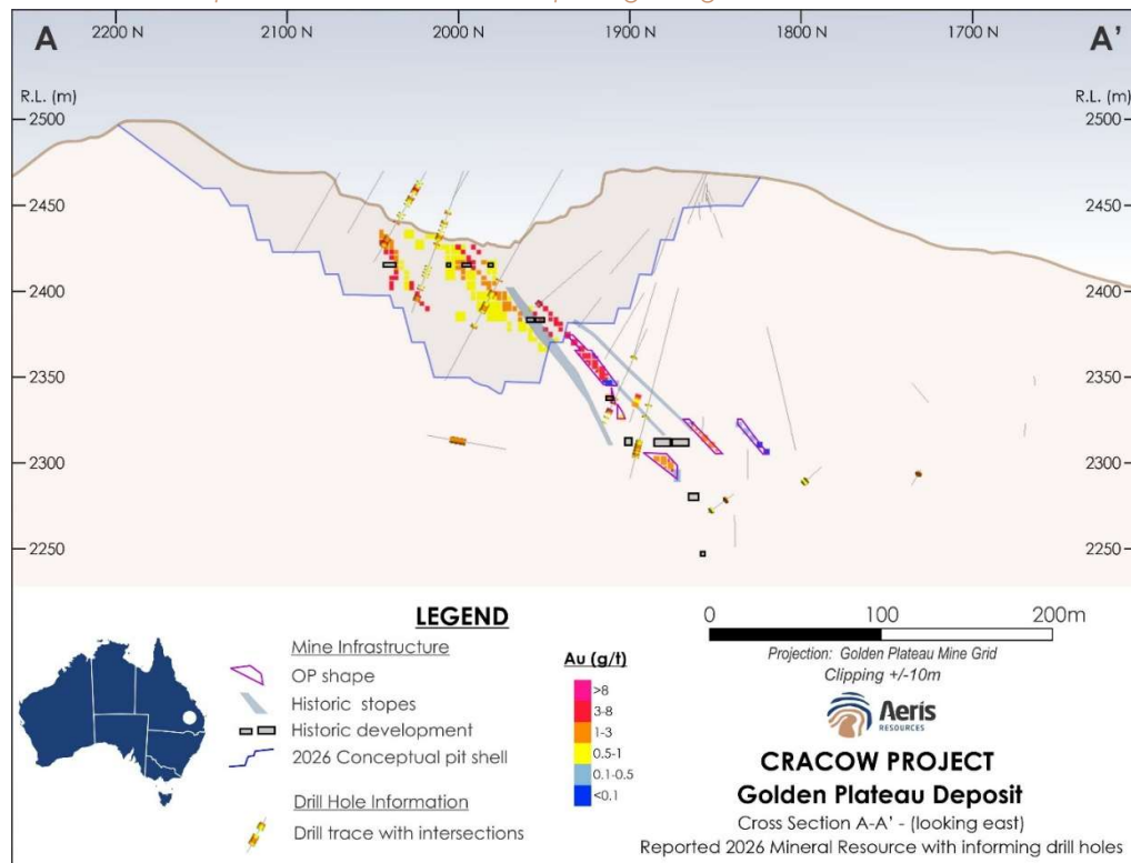
Figure 4: Cross sections through the October 2026 Golden Plateau MRE showing estimated Au grades and informing drill hole data. Note: Cross sections are displaying drill hole data +/-10m from the section plane. The block model is reporting along the section.
