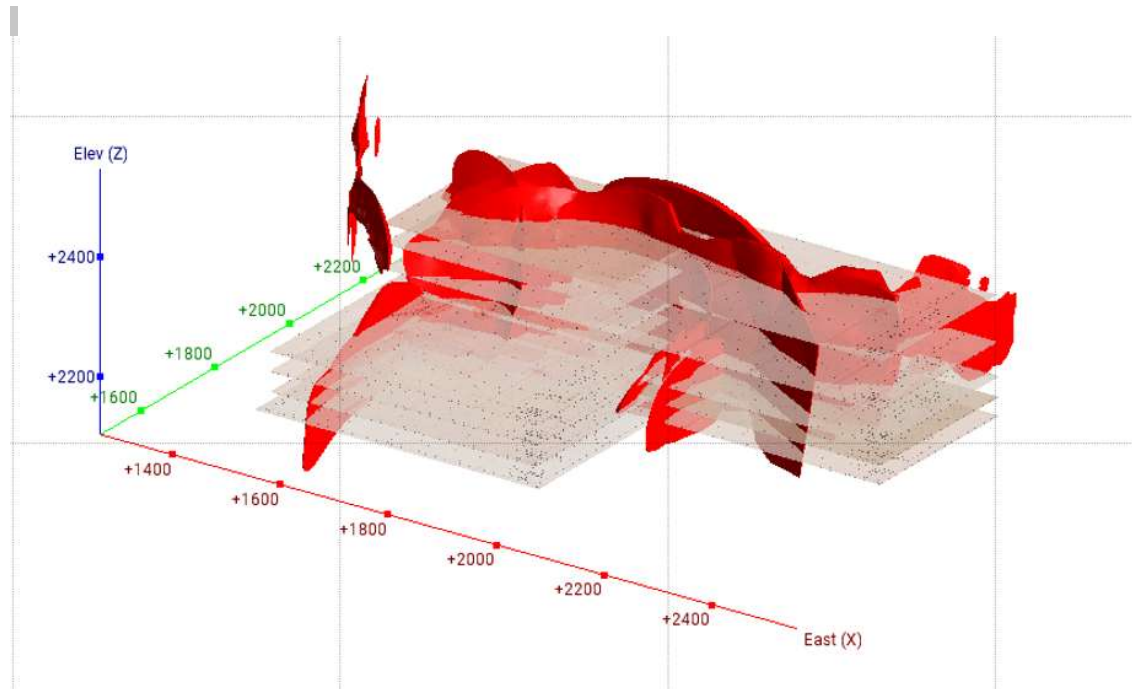
Figure 8: Oblique view northwest showing the modelled vein at Golden Plateau. Also shown are a series of historical plan view interpretations which have been used along with cross sectional interpretations (not shown).
