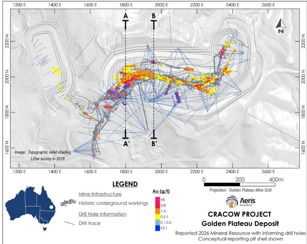
Figure 2: Plan view showing the Golden Plateau October 2026 reported Mineral Resource.
