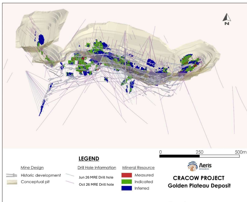
Figure 7: Oblique view looking north showing the Golden Plateau October 2026 reported MRE displayed by Mineral Resource category.
