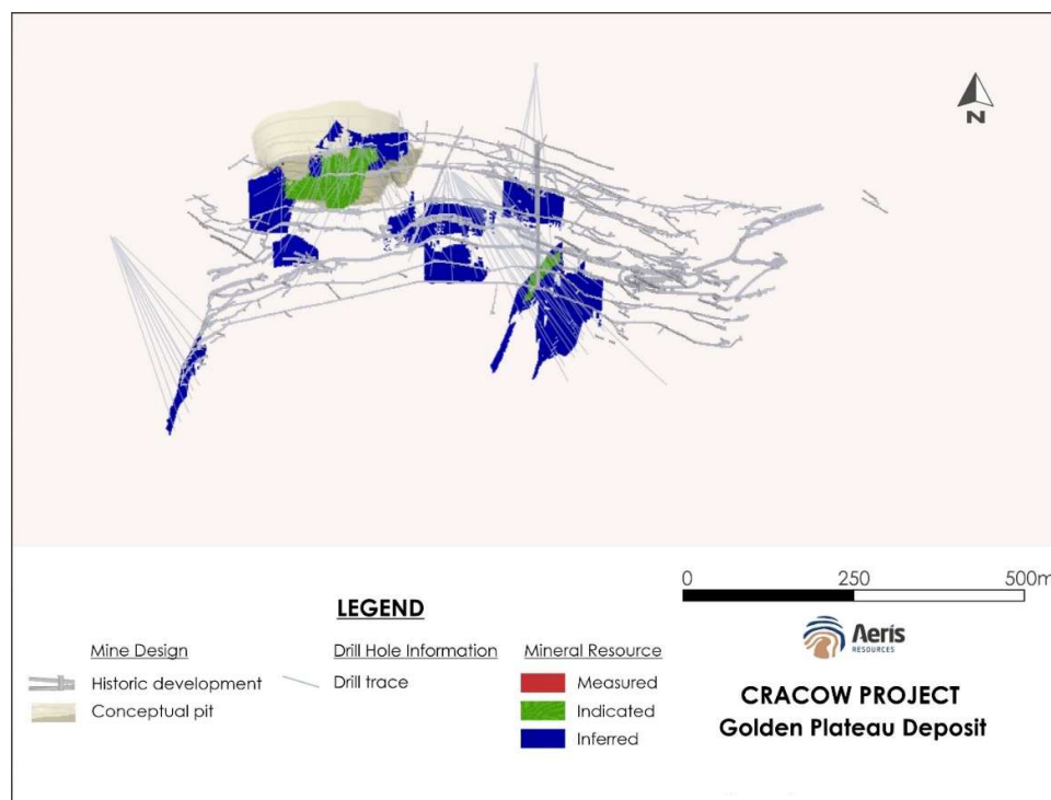
Figure 6: Oblique view looking north showing the Golden Plateau June 2026 reported MRE displayed by Mineral Resource category.
