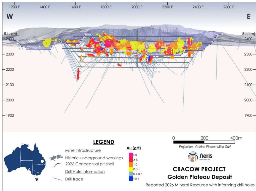
Figure 3: Long section view looking north showing the Golden Plateau October 2026 reported Mineral Resource.
