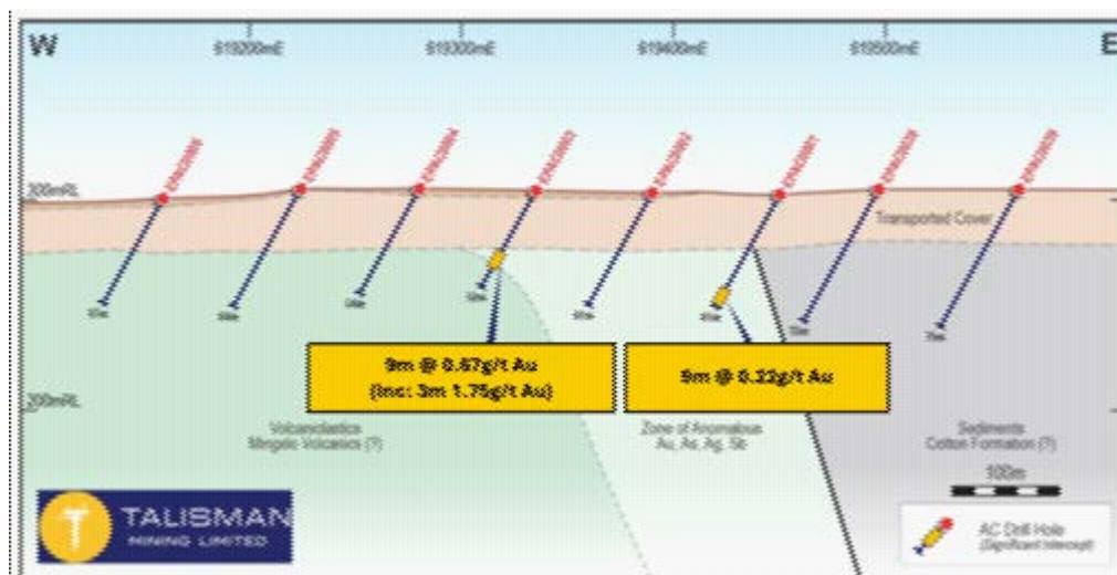
Figure 5: Cross-section of the EPH1 Target showing significant drilling results from previous Talisman drilling
