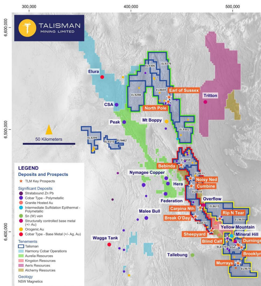
Figure 1: Talisman's Lachlan Fold Project, which covers the Mineral Hill-Canbelego Volcanic Belt (MHCVB), shown on a regional TMI Airborne Magnetic image. High-grade base metals and copper-gold deposits in the belt include CSA, Peak, Hera, Federation and Mineral Hill.
