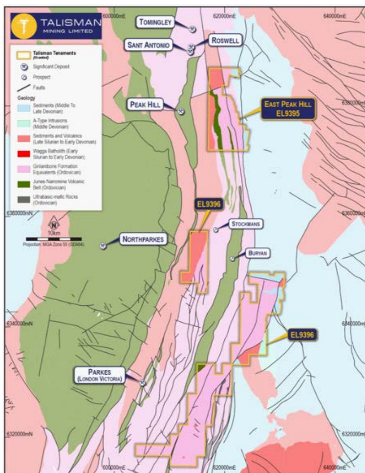
Figure 3: Regional geology plan of the Junee-Narromine Volcanic Belt illustrating the gold and copper-gold deposits of the region. Talisman tenure in the belt consists of four ELs. The East Peak Hill Project is located on EL9395, approximately 10km south-east of the Tomingley Gold Operation.
