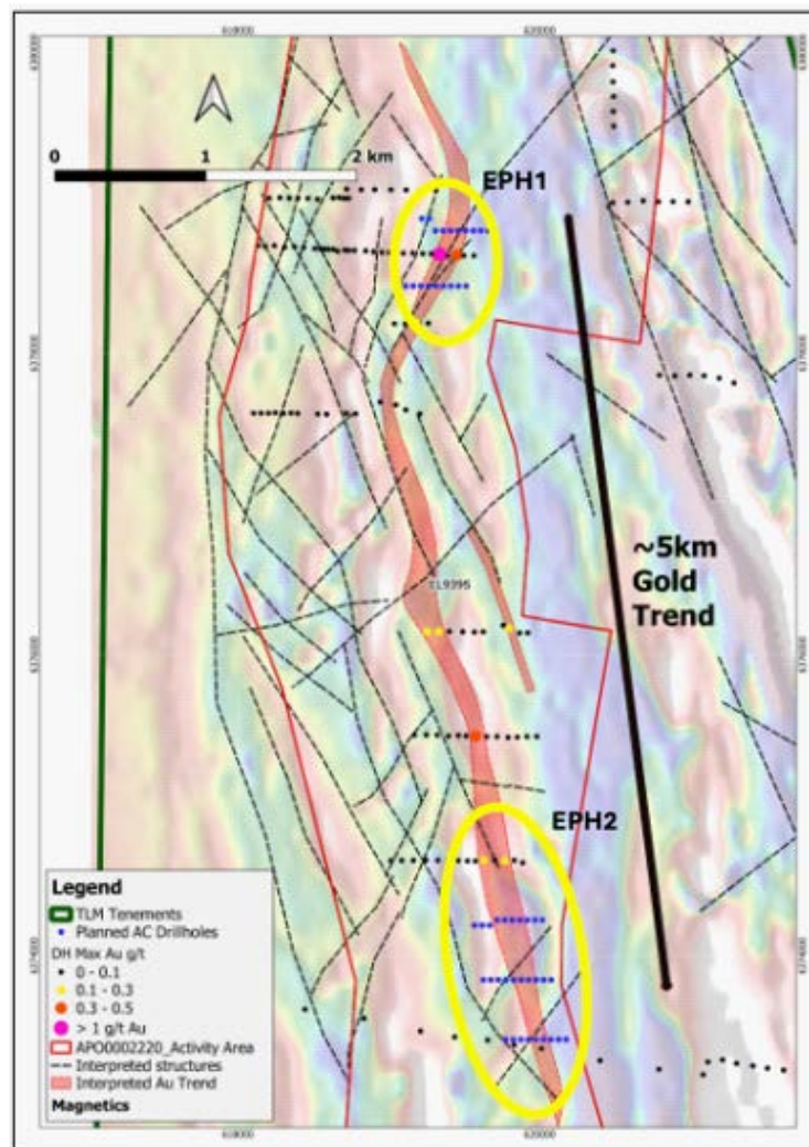
Figure 4: Target summary plan showing previous and current drill programs.
