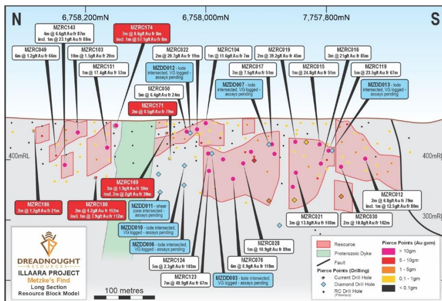
Figure 2: Long section of Metzke's Find North showing the location of drill intercepts in relation to the current Resource outline.
