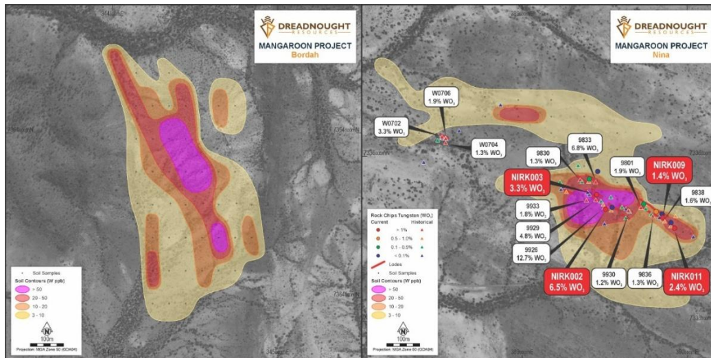
Figure 4: Plan view maps at the same scale comparing the tungsten-in-soil anomaly at Bordah (left) to Nina (right) with the Nina map showing the location of historical and Dreadnought rock chips across the “high-grade” zone.
