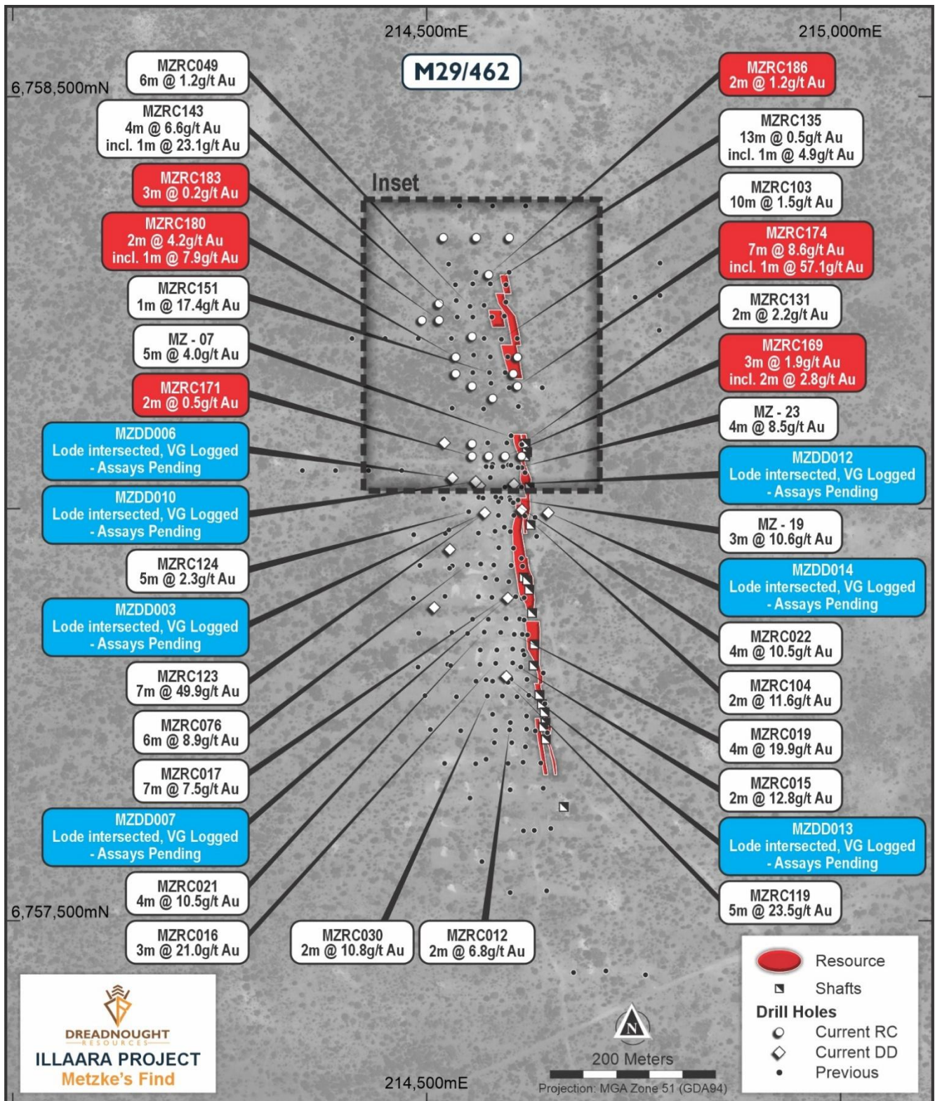
Figure 3: Plan view map of Metzke's Find and Metzke's North showing: the break in mineralisation due to a Proterozoic dyke; the location of the RC program mainly at Metzke's North (boxed area); the diamond program at Metzke's Find all in relation to previous drilling and the Metzke's Resource (24,900 oz @ 5.2 g/t Au - 84% Indicated).
