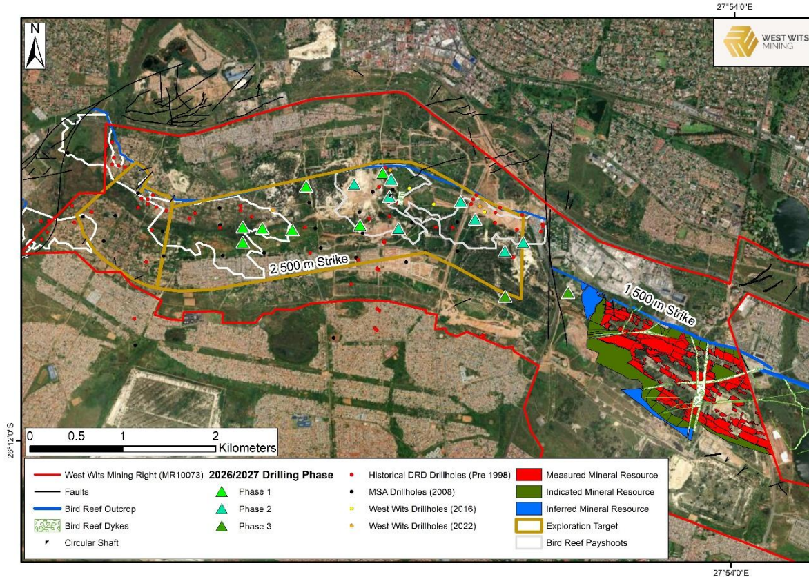
FIGURE 3: PLAN OVER TOPOGRAPHY SHOWING (1) THE MINING RIGHT (TENEMENT) BOUNDARY; (2) THE TARGET MINERALISED AREA, EXPLORATION TARGET OUTLINE AND 4,000 M STRIKE LENGTH TO BE TESTED; AND (3) PLANNED DRILLHOLE LOCATIONS BY STAGE, WITH HISTORICAL DRILLHOLES.
