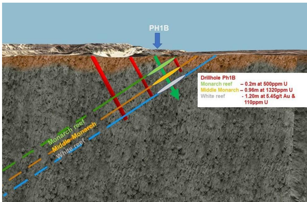
FIGURE 2: SCHEMATIC SECTION THROUGH DRILLHOLE PH1B (2022) SHOWING THE MONARCH, MIDDLE MONARCH AND WHITE REEF INTERSECTIONS. VALUES ON THE FIGURE ARE ROUNDED; SEE RESULTS ABOVE
