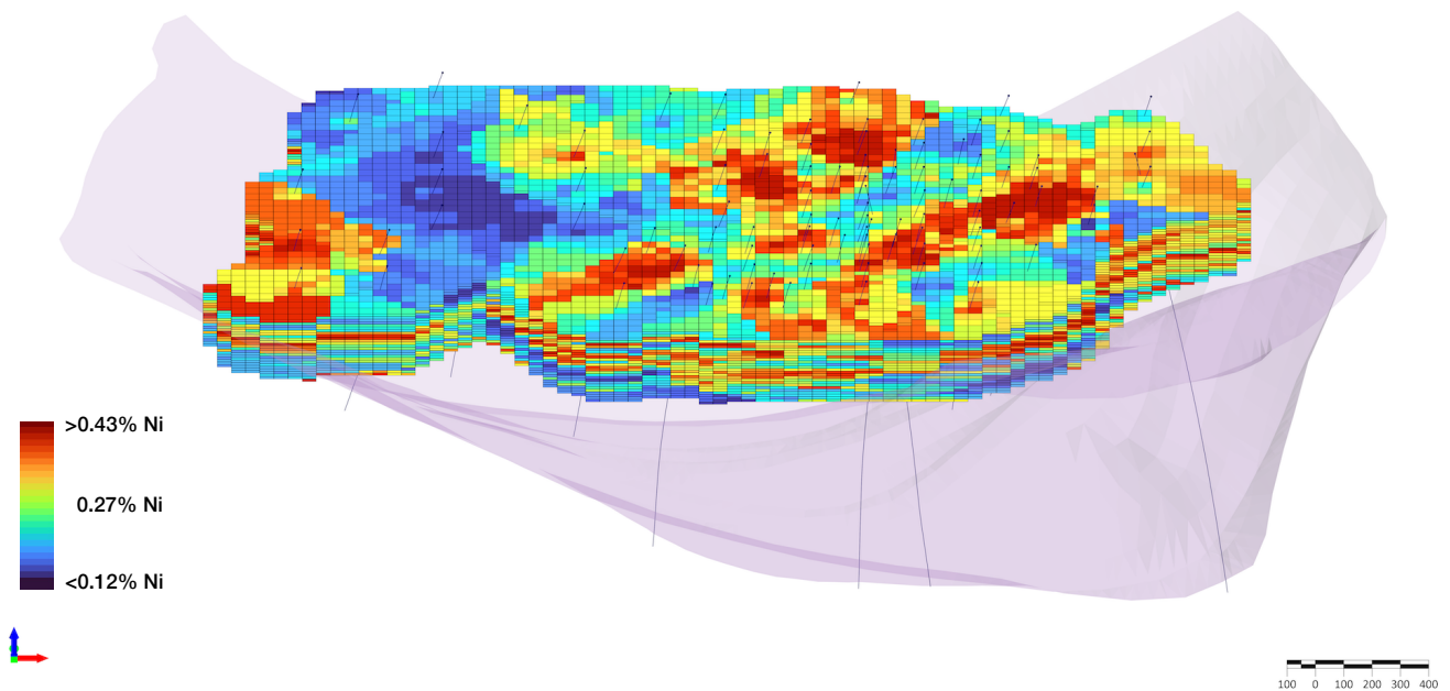
Figure 4: Mulga Tank Total Mineral Resource Block Model for the dunite domain Outline of main Mulga Tank dunite body, viewed from south looking north, coloured by Ni%
