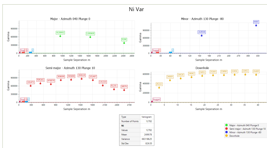
Figure 8: Variogram models for Ni
