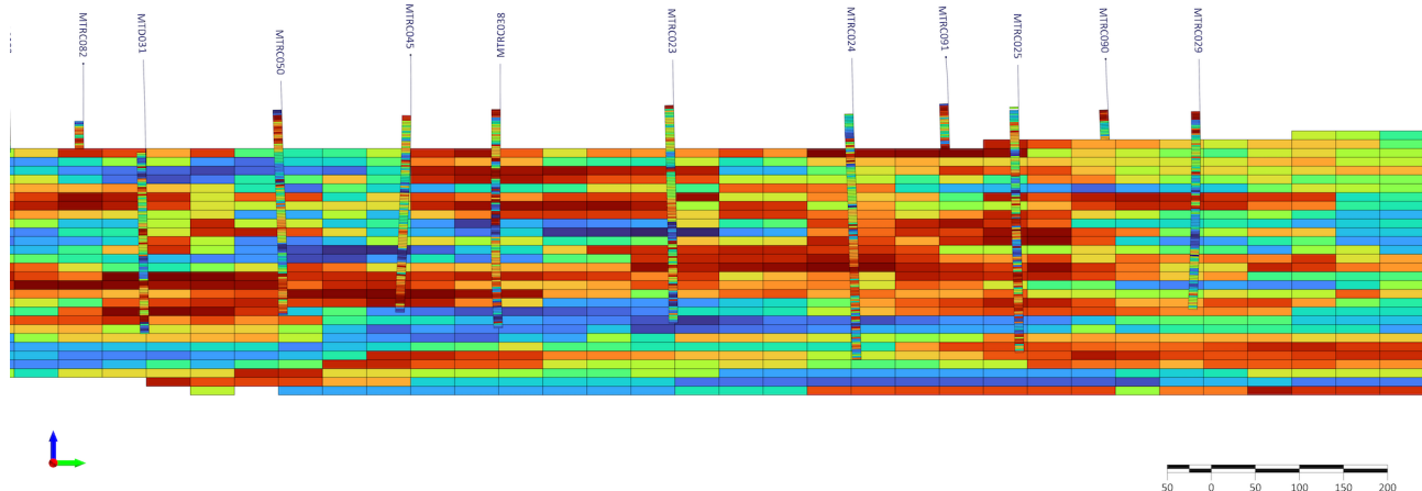
Figure 9: Visual inspection of block model and drill hole composites (section NS along E520650)
