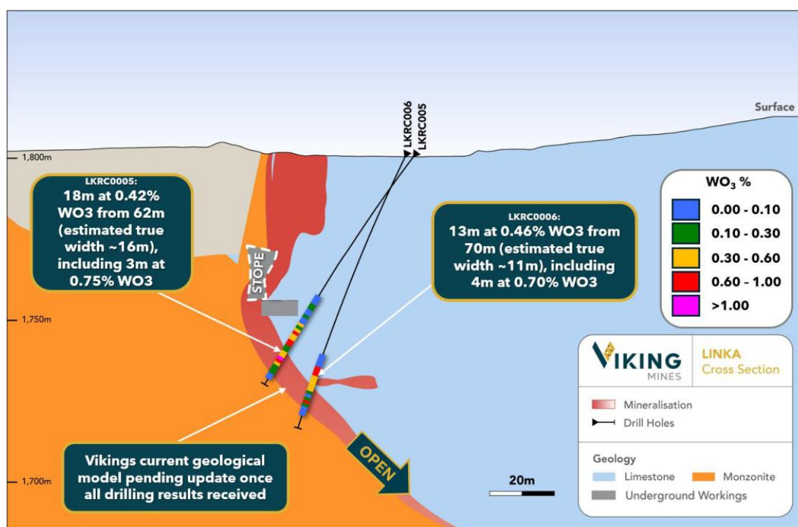
Figure 1: Cross-section through LKRC0005 and LKRC0006 showing assayed intervals relative to the modelled mineralised tactite and historical workings (looking north).
