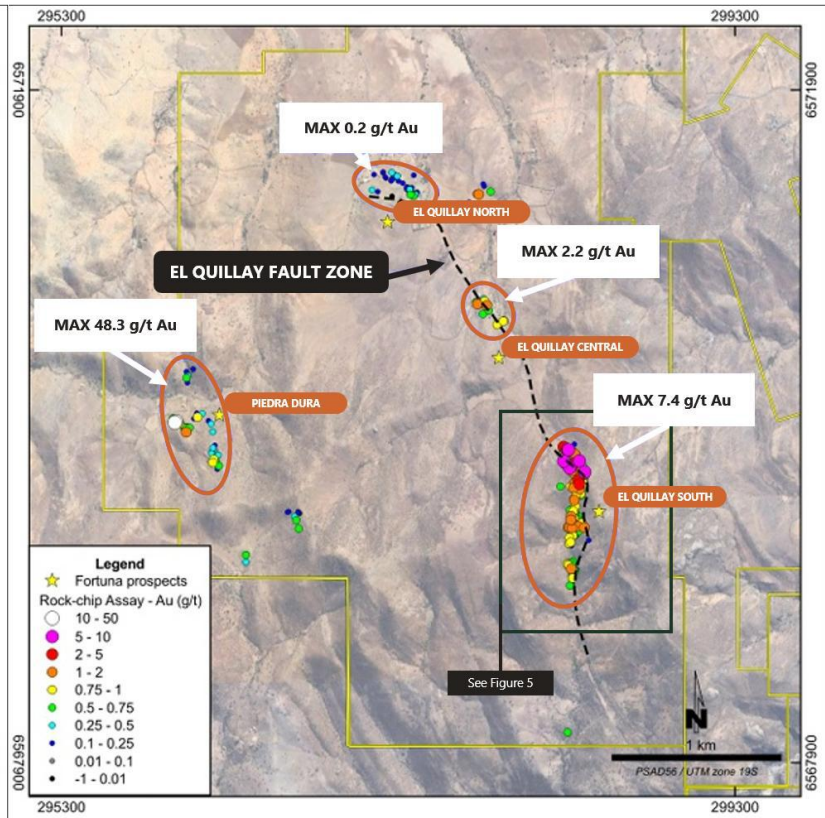
Interpreted position of the EQFZ and its association with significant gold mineralisation at various Lana Corina prospects on a satellite background
