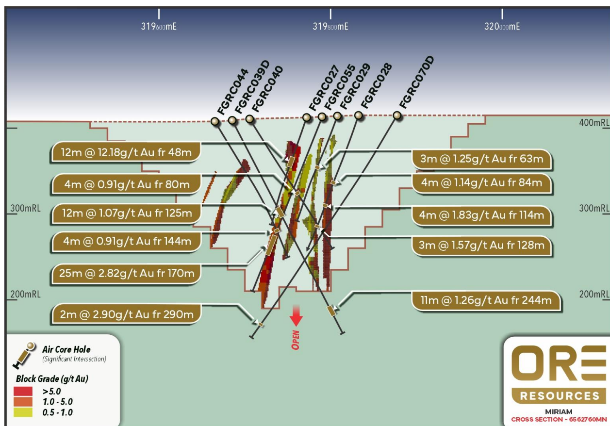
Figure 4: Forrest Prospect – Cross Section
