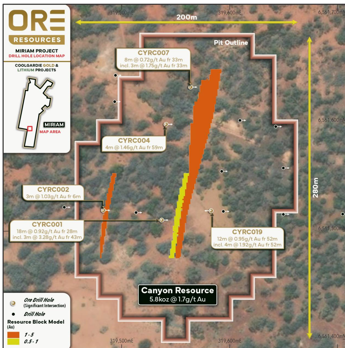
Figure 2: Canyon MRE – Plan View
