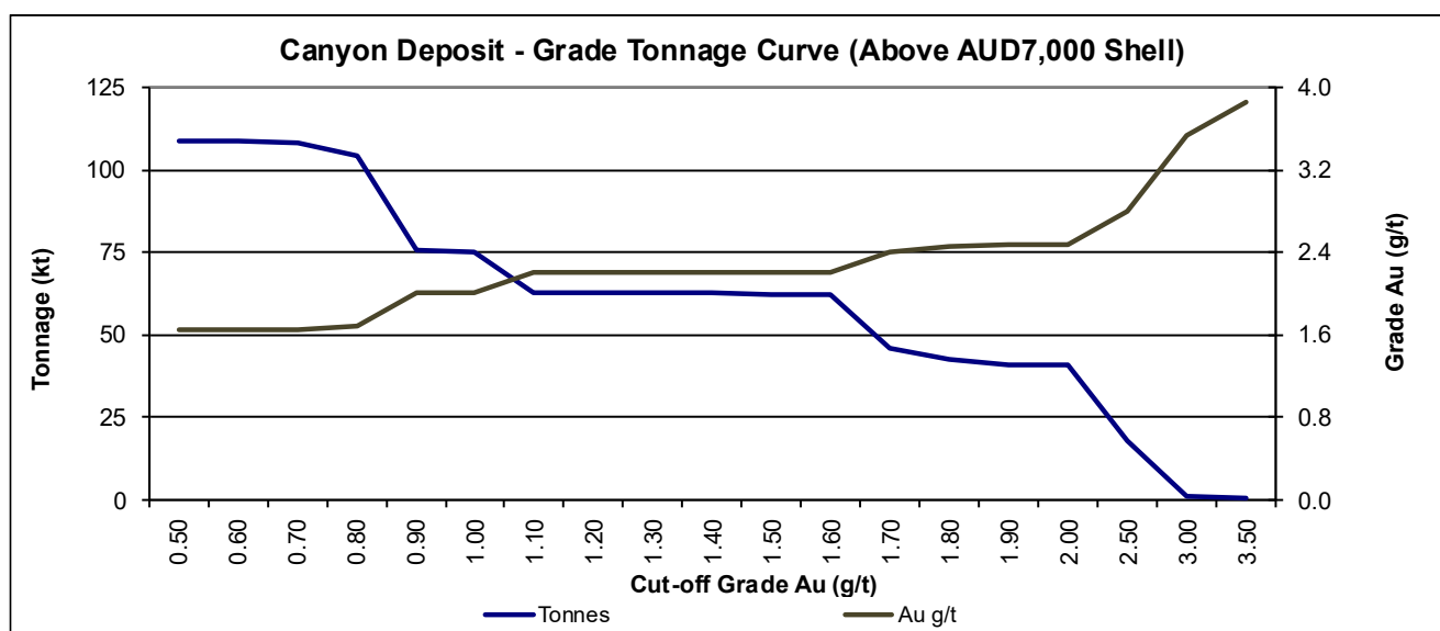
Figure 7: Canyon – Grade Tonnage Curve (above A$7,000 shell)
