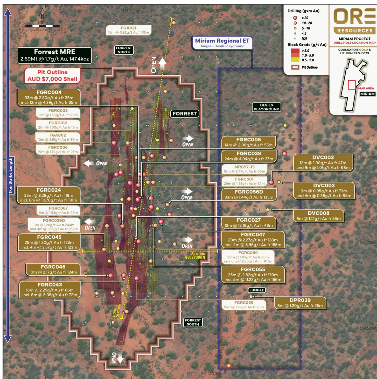
Figure 1: Forrest MRE – Plan View
