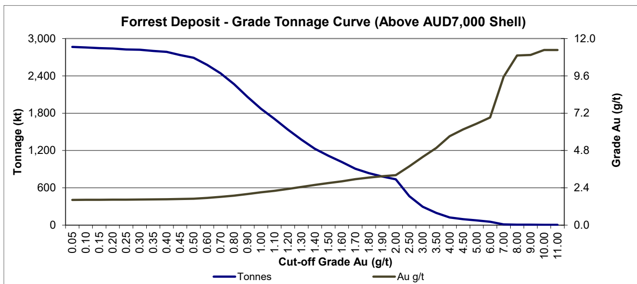
Figure 6: Forrest – Grade Tonnage Curve (above A$7,000 shell)
