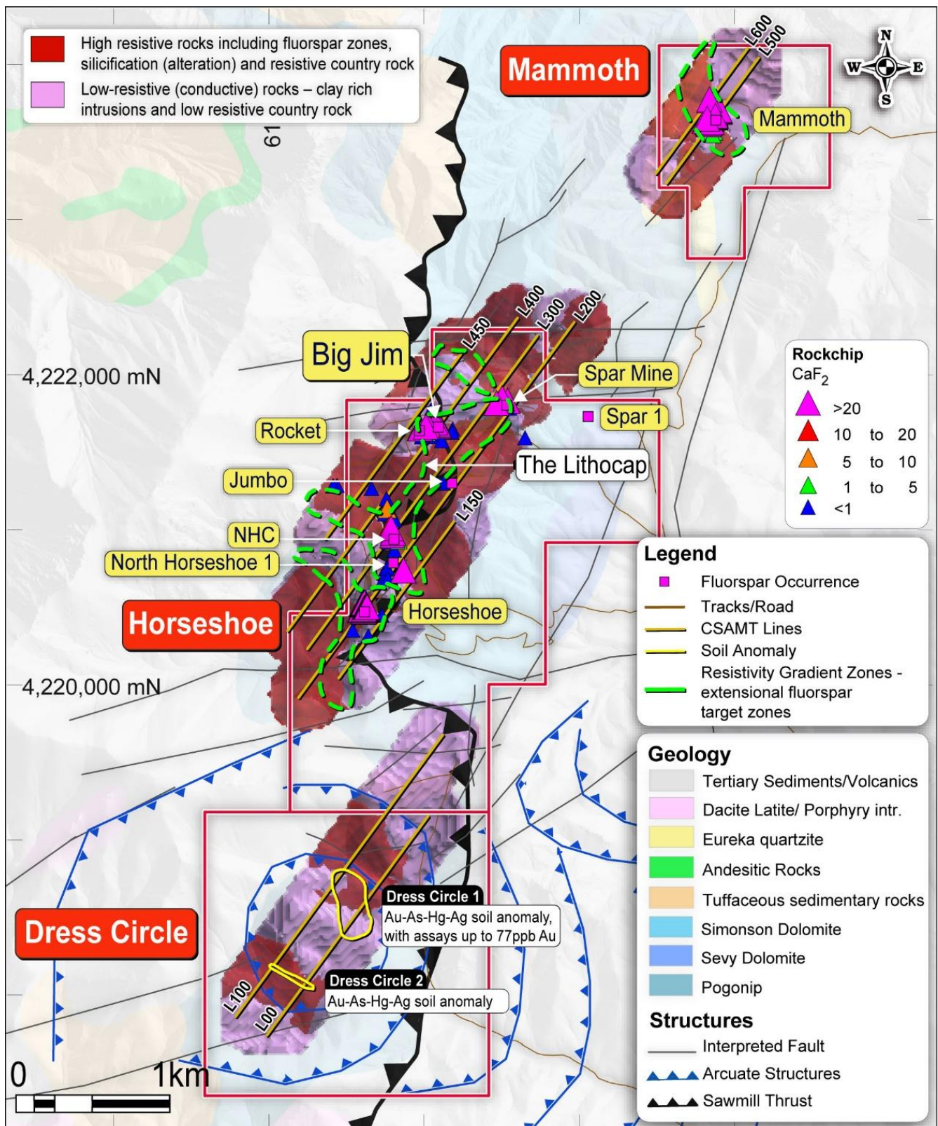
Figure 2 Map view of resistivity survey with prospect locations and transparent geology
