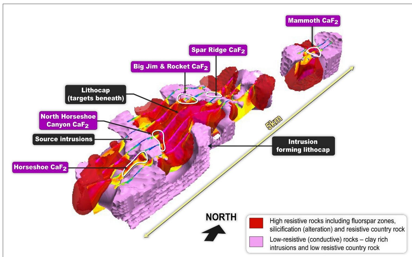
Figure 1 3D View of the CSAMT survey and modelling results
