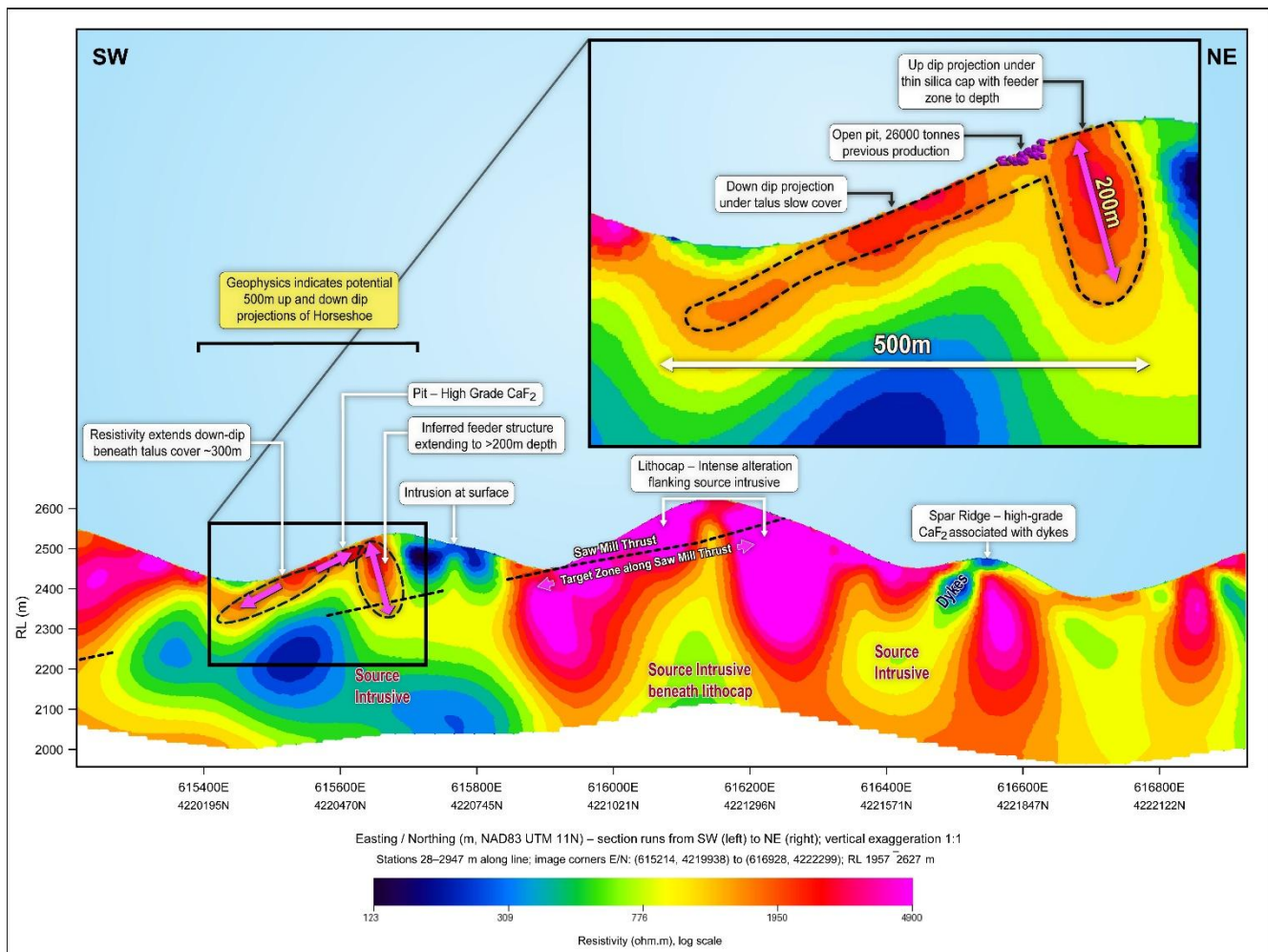
Figure 4 Section L200 from Horseshoe to the NE, indicating Feeder zone, source intrusives and the around the Lithocap
