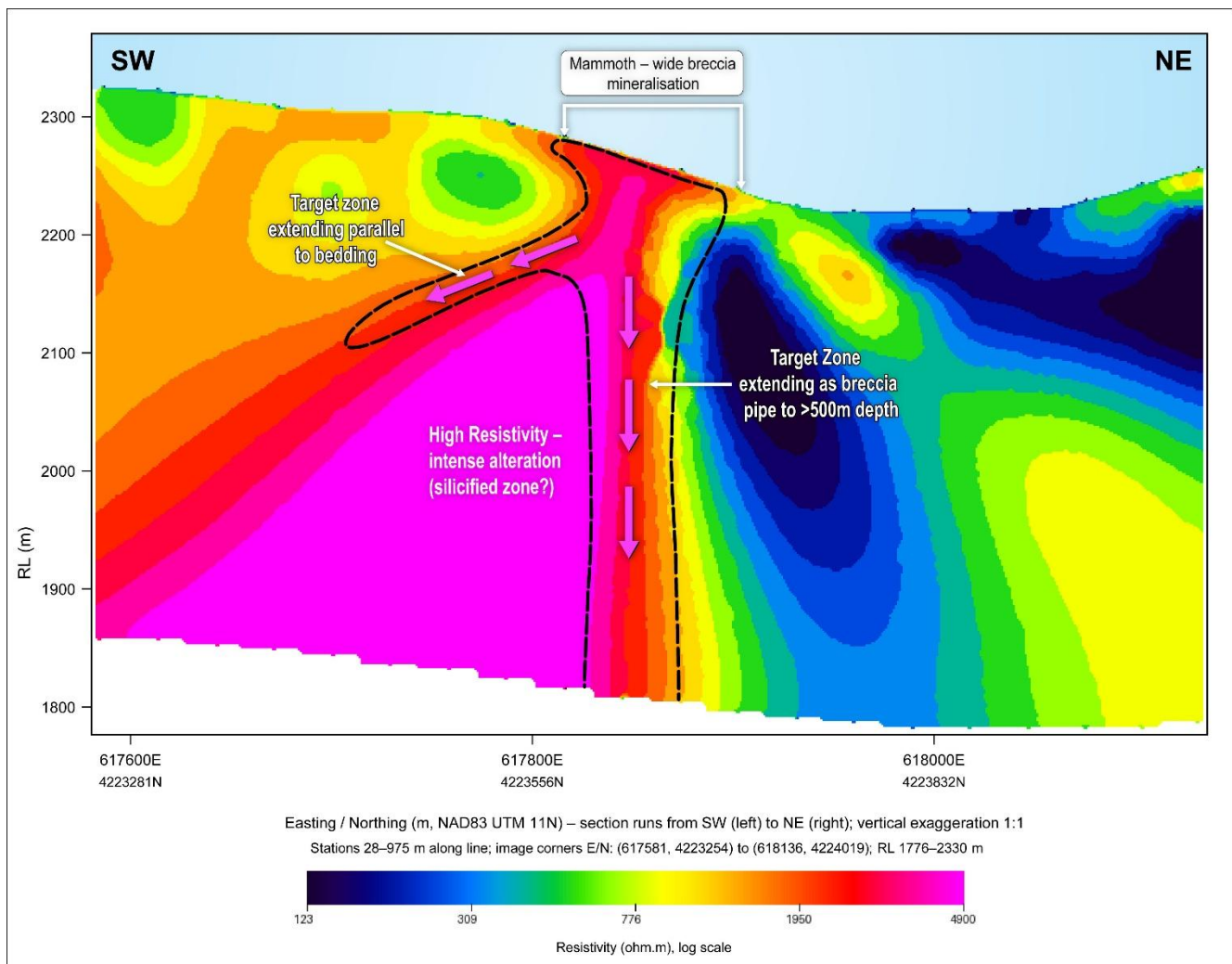
Figure 3 Section L500 CSAMT line through Mammoth
