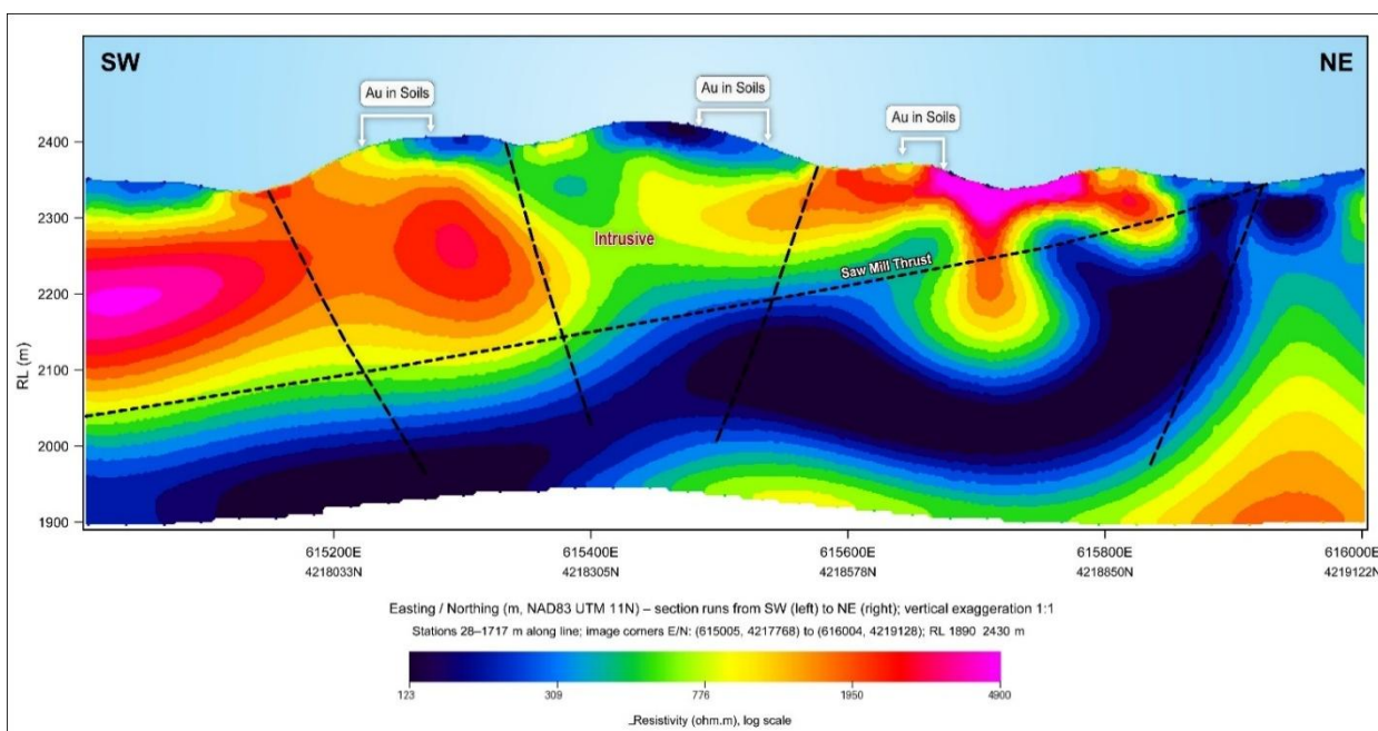
Figure 7 Section L000 at Dress Circle
