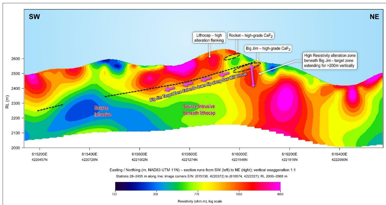
Figure 5 Section L400 from north of NW to Horseshoe through the Lithocap to Rocket and Big Jim
