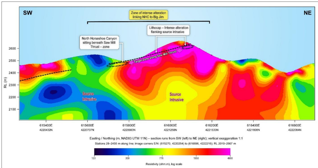
Figure 6 Section L300 from North Horseshoe Canyon, through the Lithocap to southeast of Big Jim.
