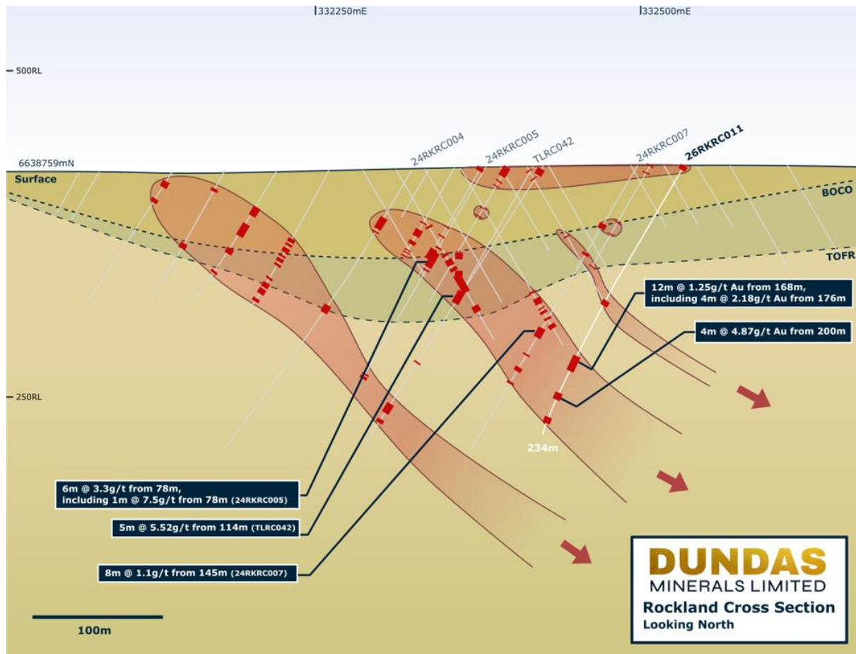
Figure 1: Interpretive cross section of the southern Rockland drill line (6638759mN, looking north). Shaded mineralised zones are interpretations (ASX: 22 September 2026)
