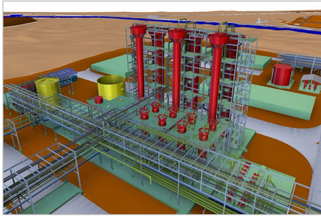
Figure 6: Model showing ion exchange area.
