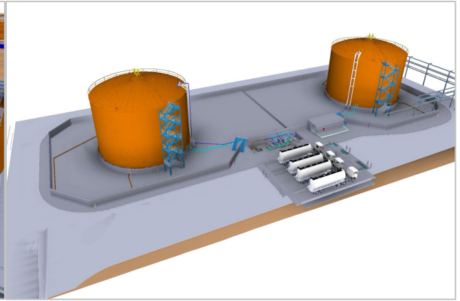
Figure 7: Model of the sulphuric acid storage area on site.
