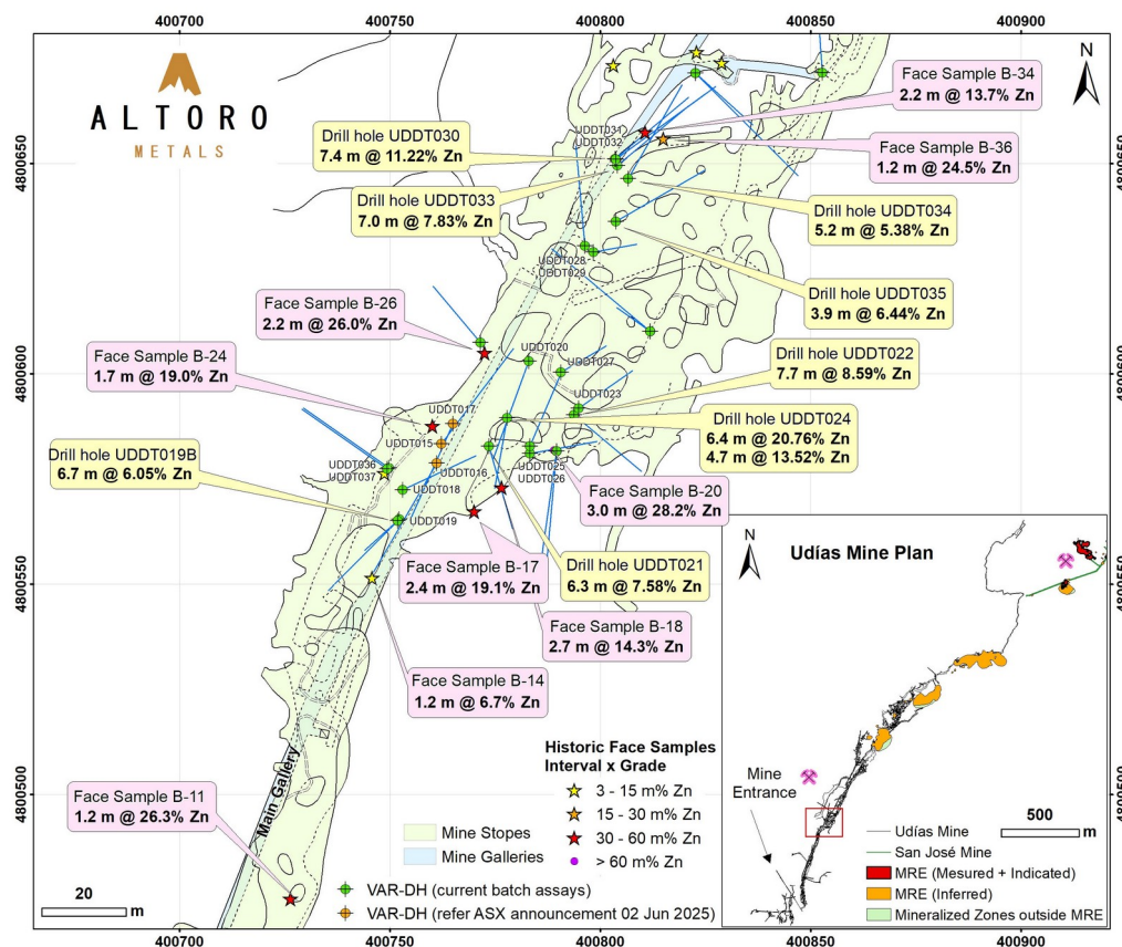
Figure 2: Plan view of the southern part of the Udías Mine showing underground diamond drillholes, mine development and historical face samples (refer ASX Announcement dated 11 November 2025)
