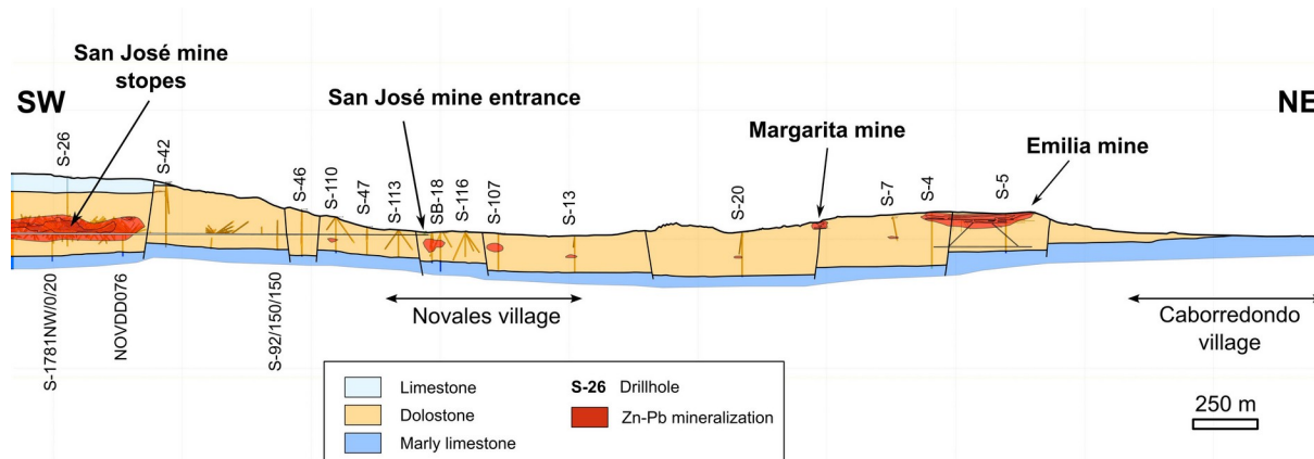
Figure 5: Simplified geological cross-section showing the continuity between the San José Mine and the Margarita and Emilia mines to the north-east
