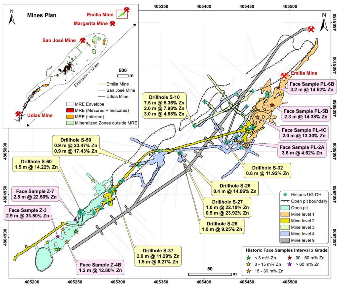
Figure 4: Plan view of historical underground drilling and face sampling results from the upper levels of the Emilia Mine (refer ASX Announcement dated 11 May 2026)
