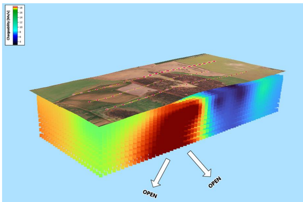
Figure 10. 3D inversion model highlighting a strong chargeability anomaly that is not closed off by the current survey coverage to the south or at depth, providing priority targets for follow-up drilling.
