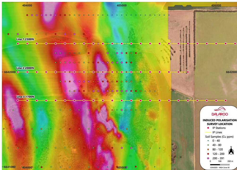
Figure 9. UAV magnetics acquired at 50 m flight altitude, overlain by Cu soil geochemistry and IP survey lines, showing the spatial relationship between magnetic anomalies, surface Cu anomalism, and IP survey coverage.
