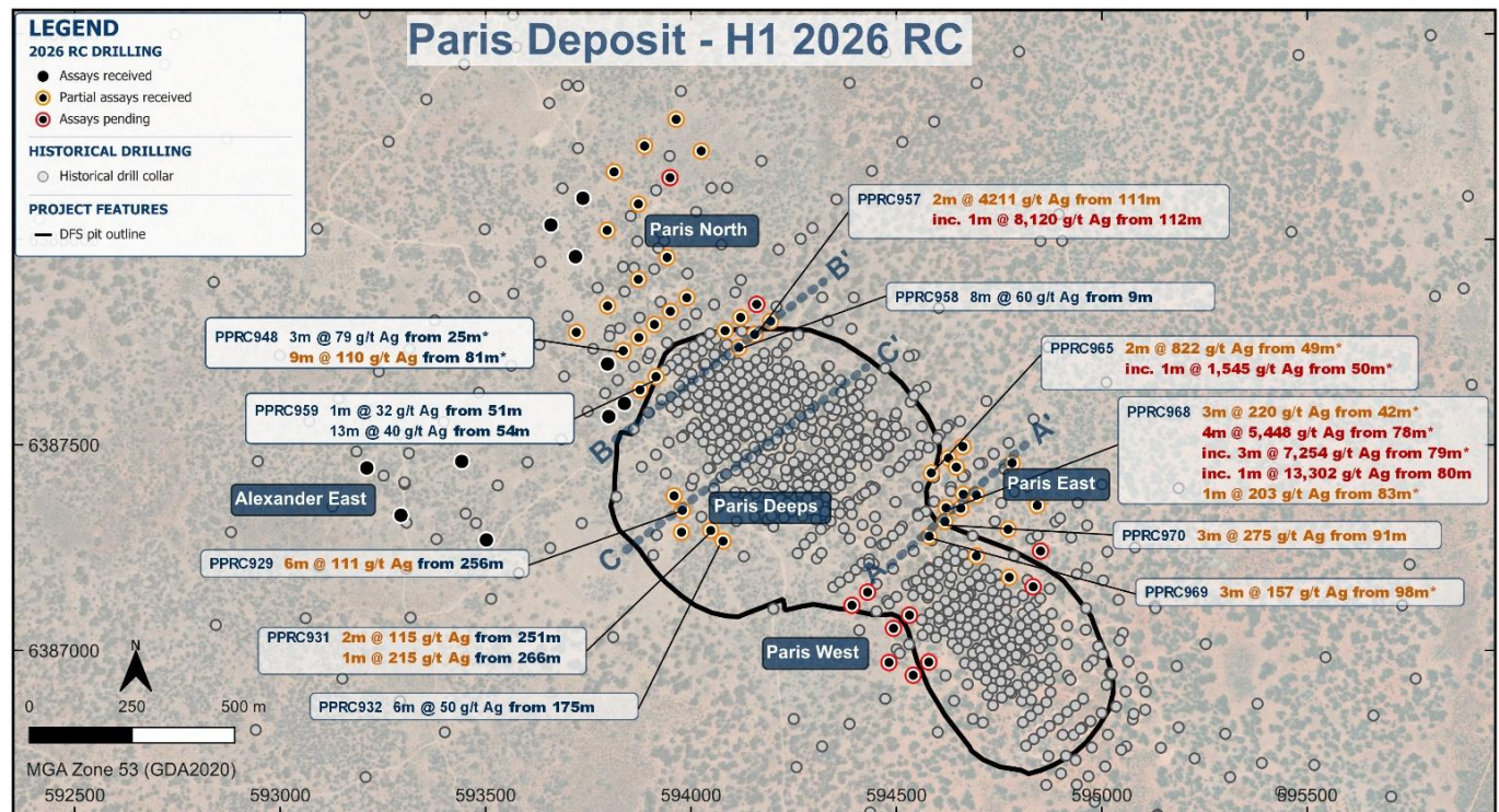
Figure 1: Paris Deposit H1 2026 RC drilling, showing historic drilling, 2026 DFS Paris optimised pit outline, main targets and key results to date. cross-sections annotated for reference. Shown on satellite true colour image.
