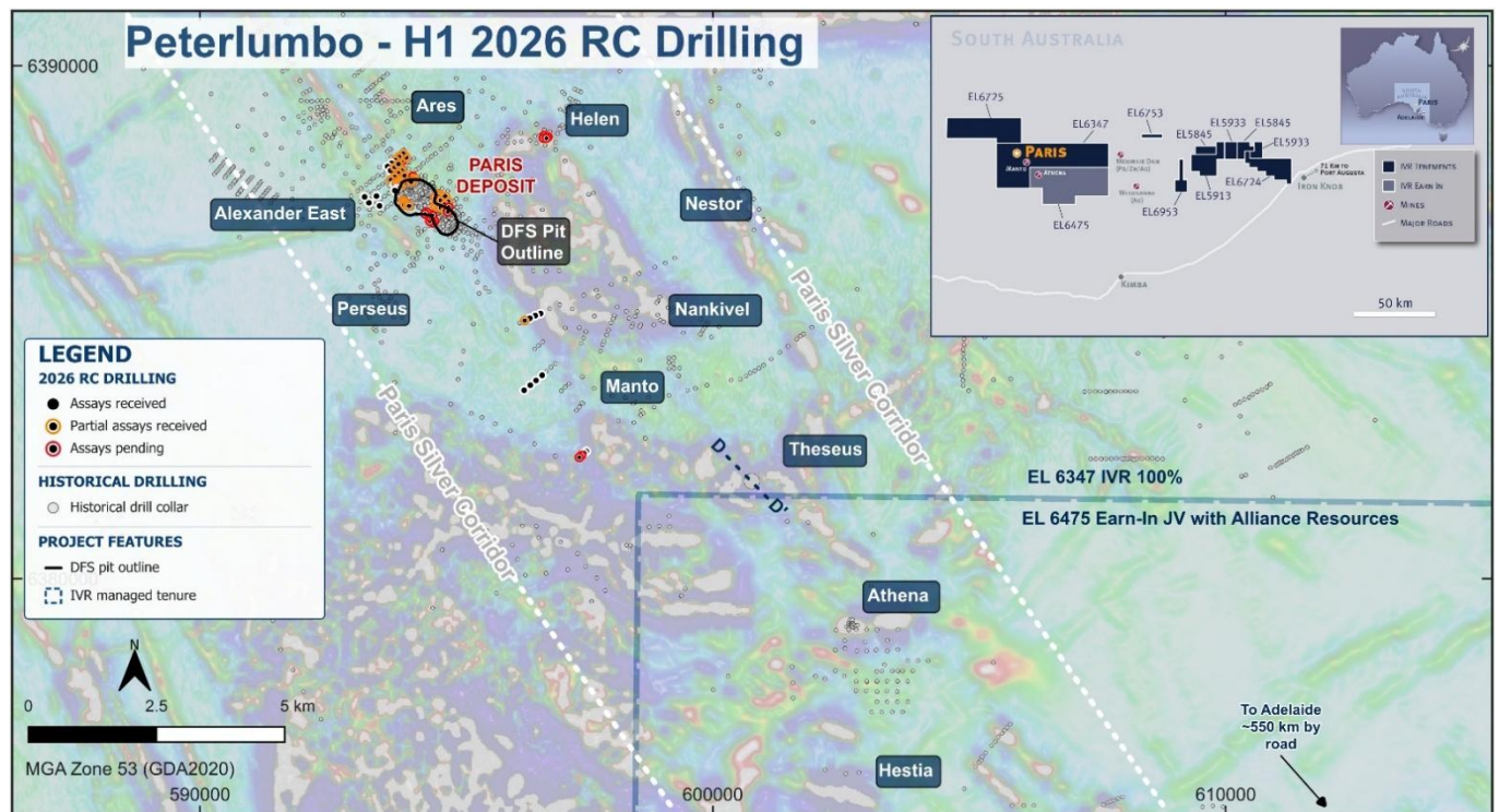
Figure 2: H1 2026 RC drilling, showing historic drilling, key regional targets, 2026 DFS Paris Deposit pit outline, tenure, the Paris Silver corridor, and Theseus cross-section location. Shown on coloured 1VD AMAG image.
