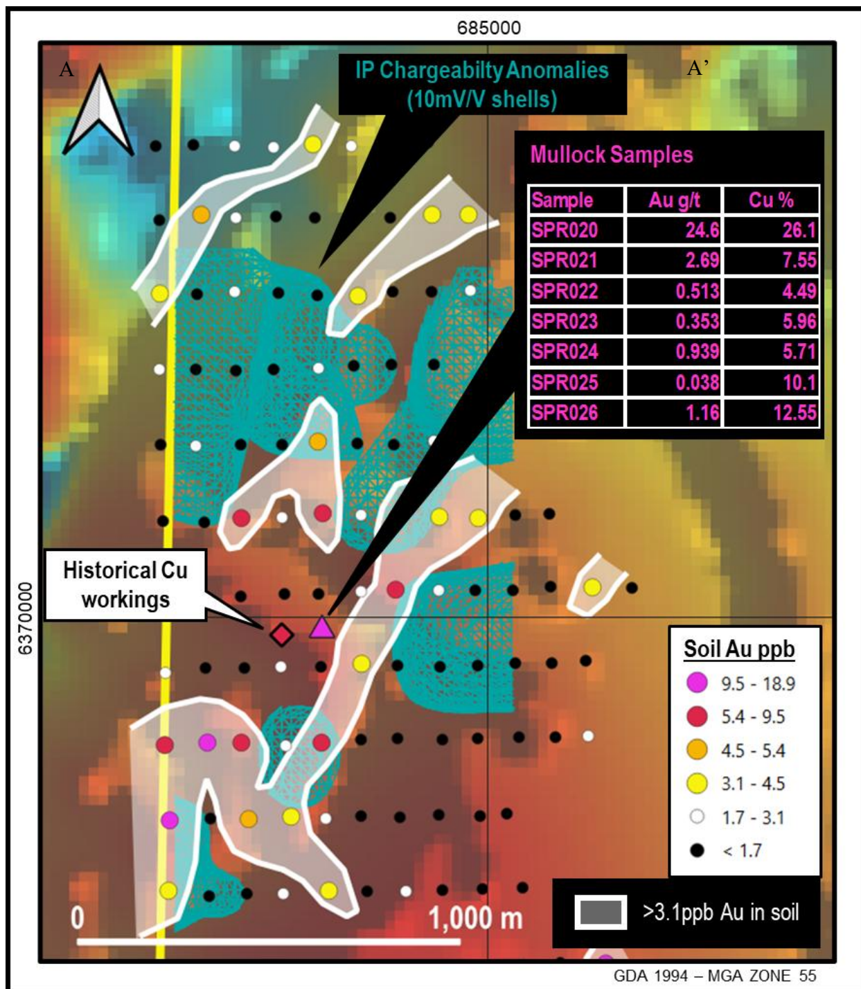
Figure 5: Total magnetic intensity (TMI) image over Gowan Green, showing Au-in-soil results and an earlier IP chargeability features that are currently under review. Copper and gold values for mullock samples collected from the historical copper workings are also shown. Further analytical results for these samples are provided in Table 1 (Refer ASX: SLZ 20 May 2020).
