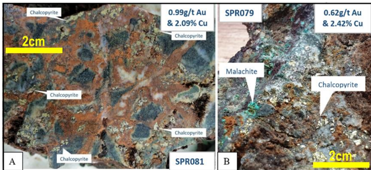
Figure 8: Samples of mineralised chalcopyrite- and malachite-bearing skarn breccia from Razorback-Wattle Ridge. Both samples were collected close to the collar location of RZD001. The sample locations are provided in Table 2.
