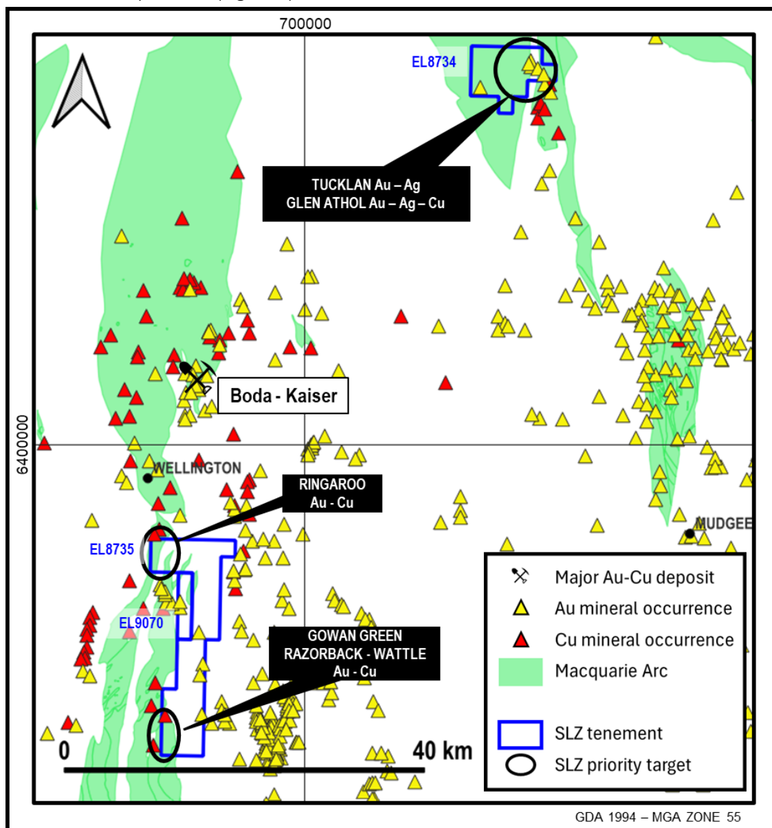
Figure 2: SLZ's LFB tenements and priority target areas relative to the mapped exposures of the Macquarie Arc, gold and copper mineral occurrences from the Geological Survey of NSW database and the Boda-Kaiser porphyry Au-Cu deposit.
