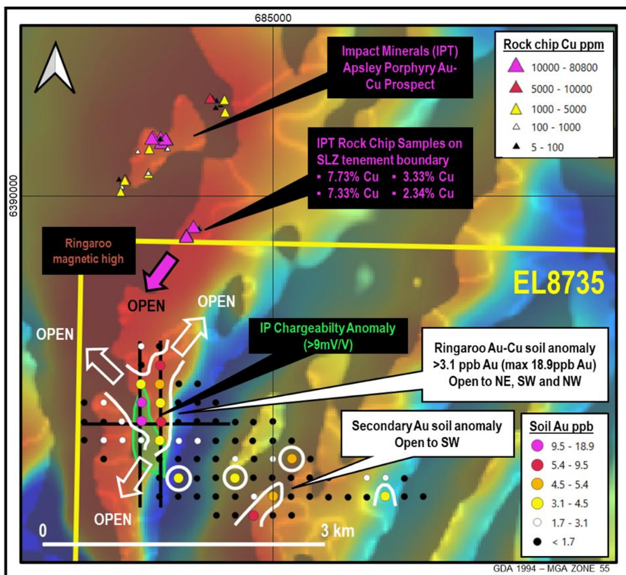
Figure 3: Total magnetic intensity (TMI) image over Ringaroo showing soil sample coverage and gold results, IP lines (black) and the IP chargeability anomaly, and Impact Minerals rock chip results from the Apsley porphyry prospect (ASX: IPT 14/01/2020 & 23/04/2020) immediately north of EL8735 (ASX: SLZ 9 July 2020).
