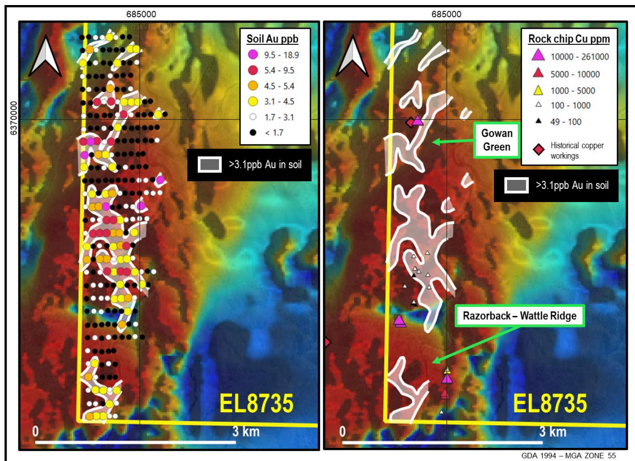
Figure 4: Total magnetic intensity (TMI) image over the Big Hill area, showing (left) gold-in-soil results, with anomalous >3.1ppb Au values contoured; and (right) rock chip copper values relative to the anomalous soils, the location of the historical workings at Gowan Green, and the locations of the Gowan Green and Razorback-Wattle Ridge targets. The central portion of the soil anomaly corresponds to the Big Hill target. Note that due to the narrow focus of the soil survey, most of the anomalous zones remain at least partially open to the east. The magnetic high corresponding to the Molong Volcanic Belt is clearly visible (ASX: SLZ 30 September 2020).
