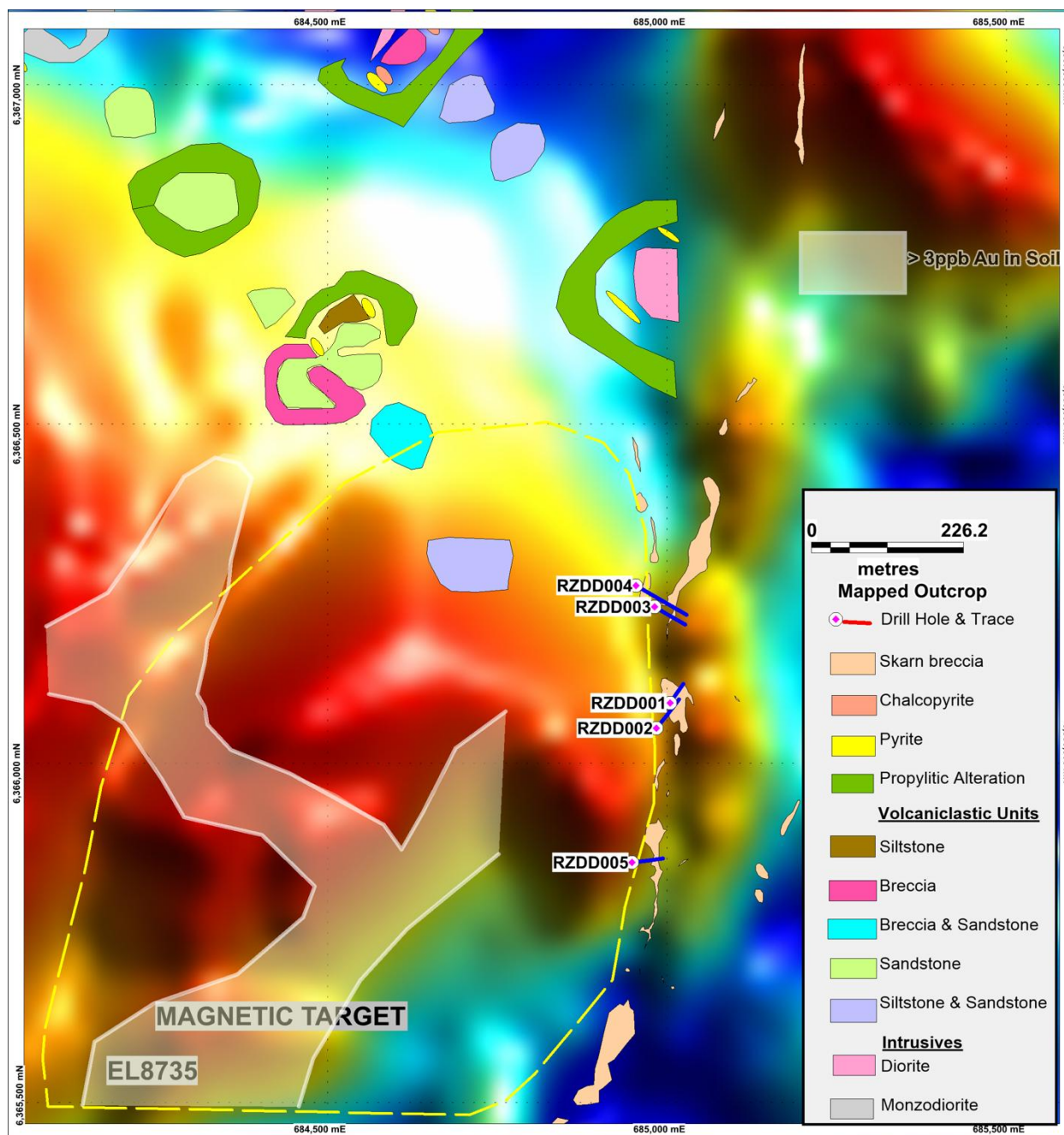
Figure 7: Total magnetic intensity (TMI) image over Razorback-Wattle Ridge showing the mapped surface lithology, magnetic target and previous drilling, which focused on the mapped surface skarn breccia. The dashed yellow line shows an interpreted possible porphyry target based on the magnetics and previous drilling results, with the skarn breccia located along its eastern margin. (Refer to ASX: SLZ 3 February 2022 and ASX: SLZ 15 March 2022).
