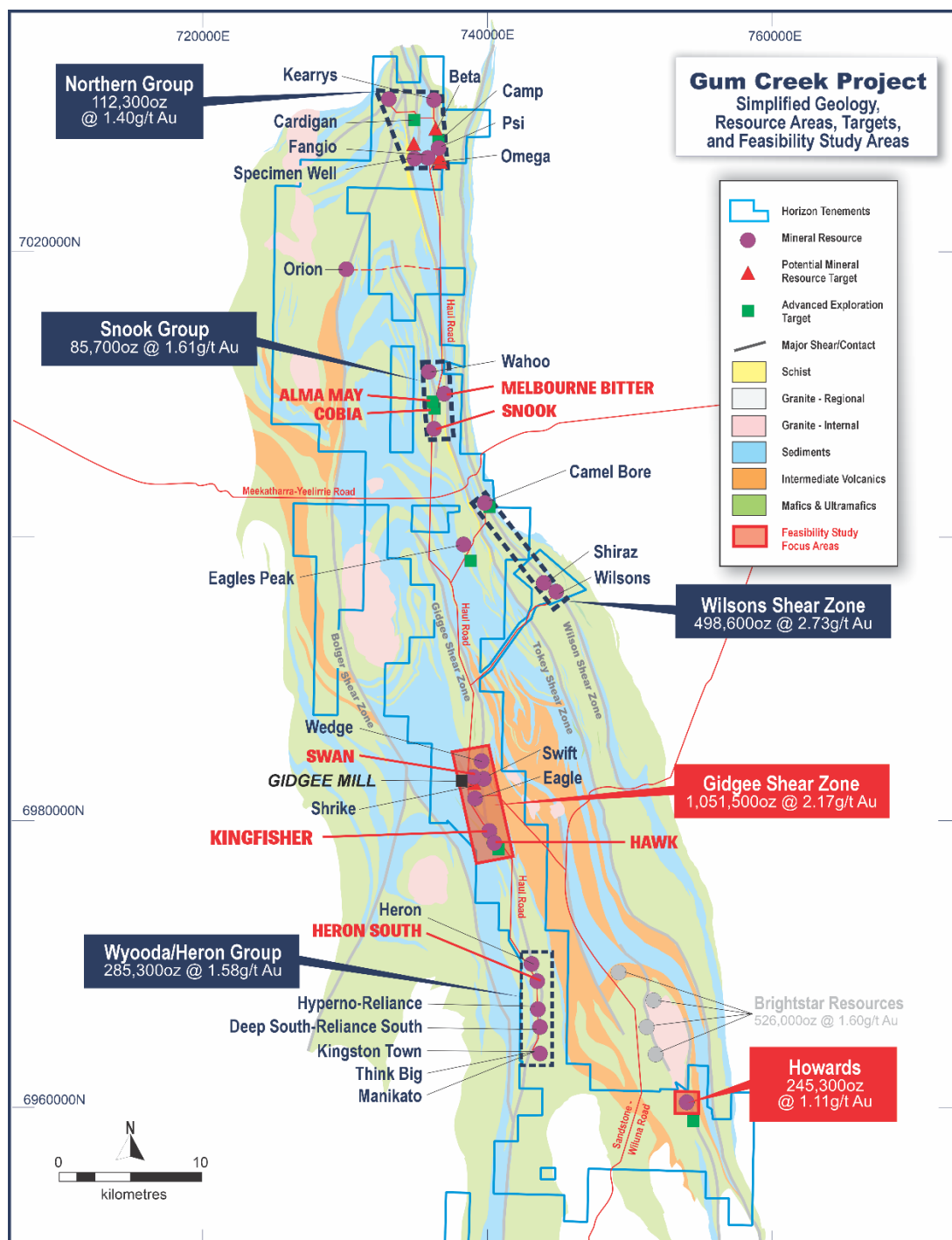
Figure 2: Gum Creek Gold Project existing Mineral Resources, Potential Mineral Resources and Exploration Targets over simplified geology.
