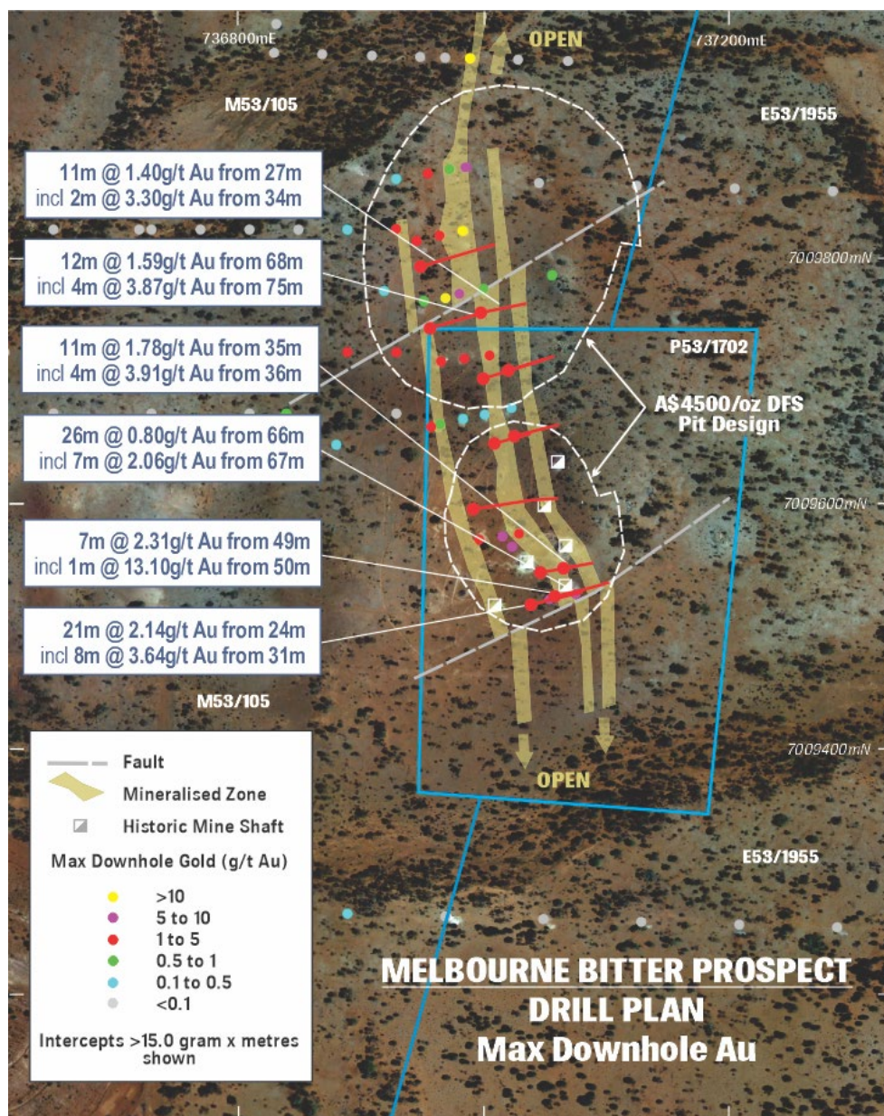
Figure 9: Melbourne Bitter drill hole plan showing all drill collars coloured by maximum downhole gold (g/t) and recent gold intercepts over satellite image.
