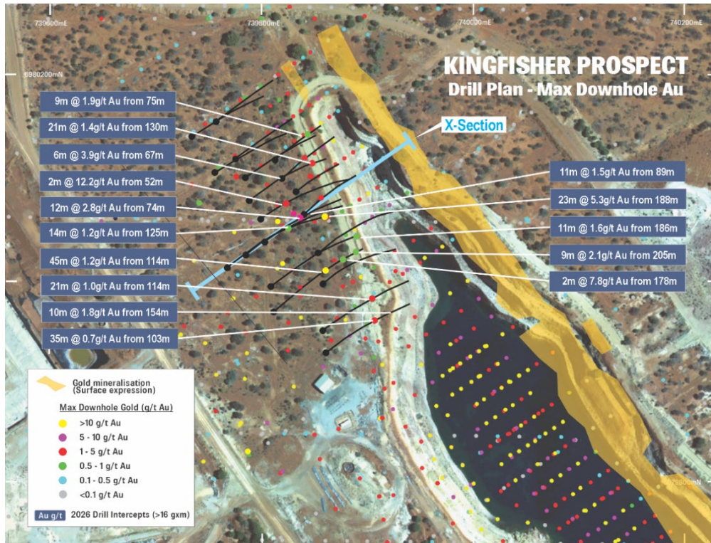
Figure 5: Kingfisher drill hole plan showing all drill collars coloured by max. downhole gold (g/t) and recent drill hole gold intercepts over satellite image.
