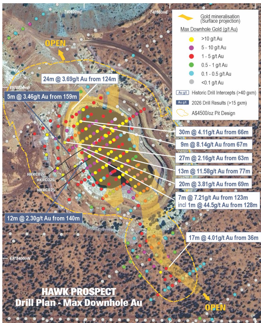
Figure 12: Hawk drill hole plan showing all drill collars coloured by maximum downhole gold (g/t Au), recent gold intercepts and historic intercepts (>40 GxM) over satellite image.
