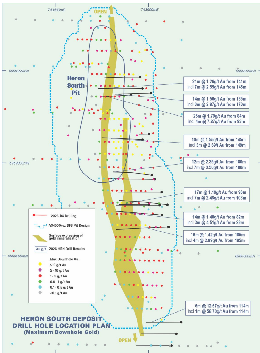
Figure 8: Heron South drill hole plan showing all drill collars coloured by maximum downhole gold (g/t) and recent drill hole gold intercepts.
