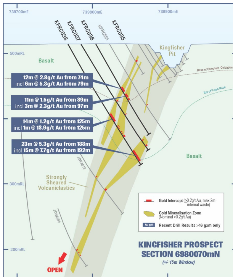
Figure 6: Kingfisher cross section showing recent RC drilling intercepts, interpreted geology and Kingfisher open pit.
