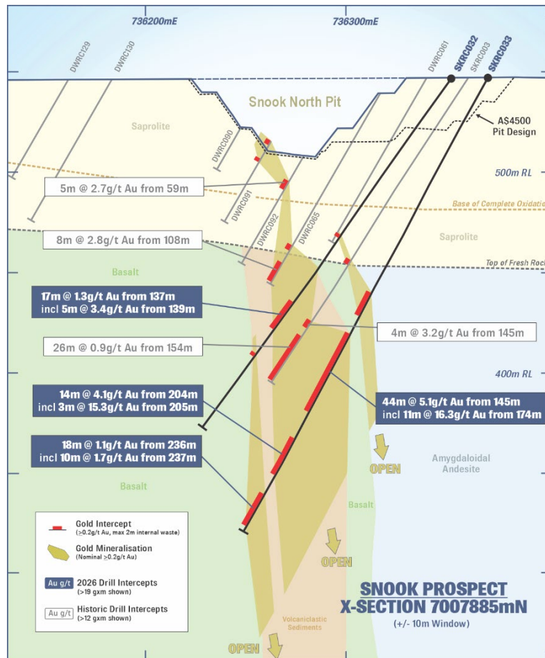
Figure 4: Snook cross section showing interpreted geology, mineralised zones and recent significant drill intercepts.
