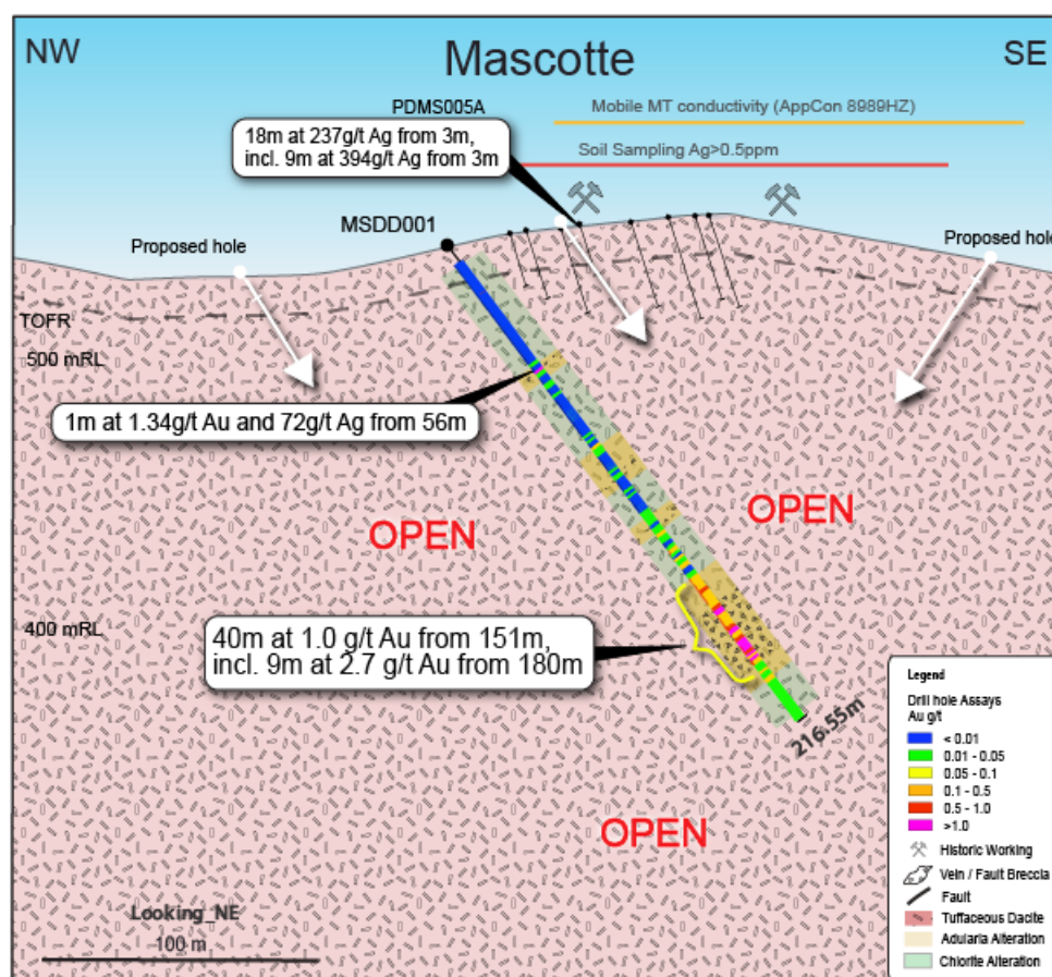
Figure 2. Section view of the Mascotte Silver-Gold Prospect - MSDD001 drill hole showing completed and planned drill holes.
