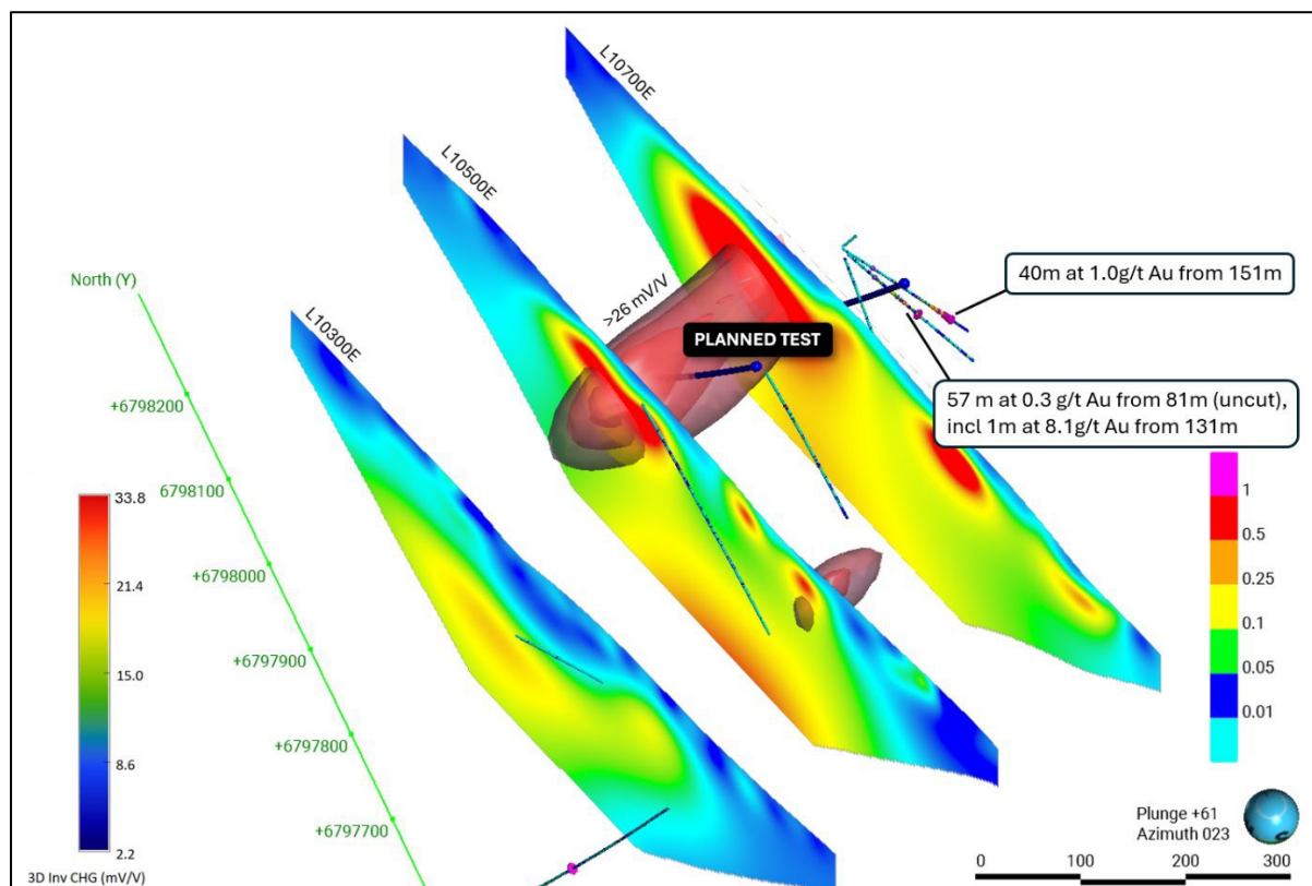
Figure 3. Oblique 3D view (looking northeast) of the Mascotte DDIP 2D inverted chargeability sections with 3D chargeability iso-shells (26mV/V and higher). Drill holes shown are the 2025-2026 LGM drilling.
