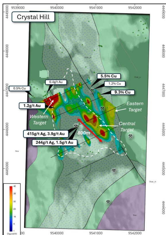
Figure 6. The Crystal Hill magnetic low target area (white dashed line) with 3D inverted chargeability iso-shells over highlight rock chip assays, historic workings and geology. xxvi
