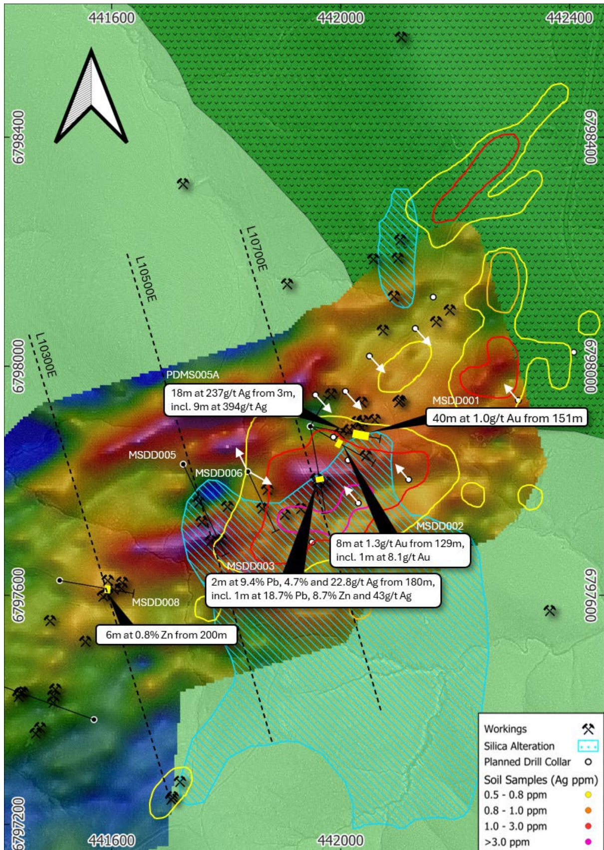
Figure 4. Mascotte historic drill results and soil sample contours (Ag ppm) over GAIP chargeability.
