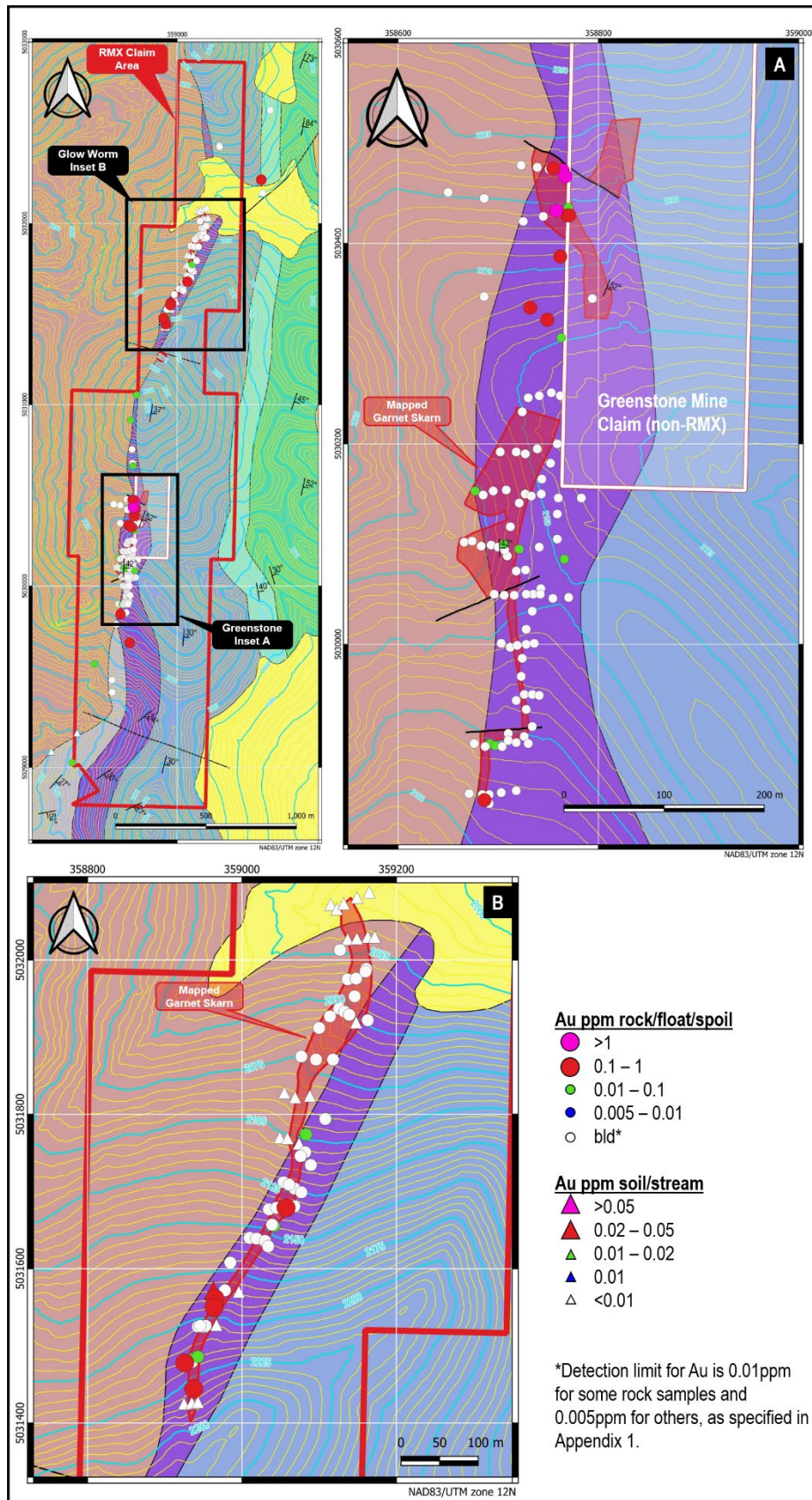
Figure 8: Gold (Au) results for the Greenstone and Glow Worm prospects relative to topography and USGS surface geology after McDonald and Yakovlev (2019) 29 and mapped garnet skarn after Pattee (1960) 30 . For geology legend refer to Figure 3.
