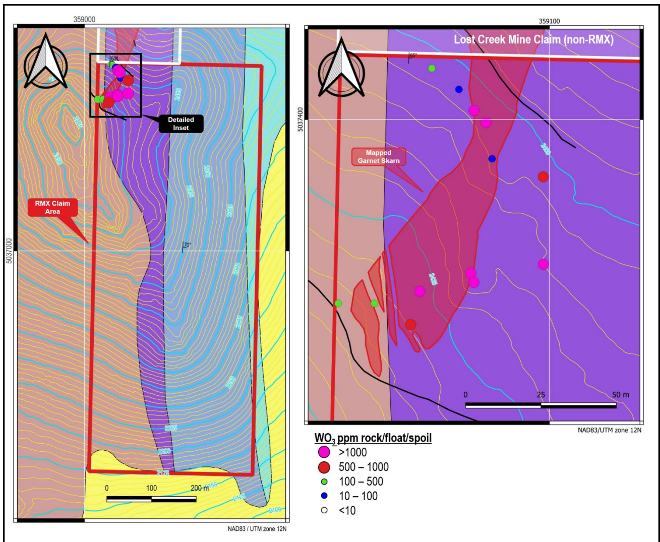
Figure 5: \text{WO}_3 results for the Lost Creek prospect relative to topography and USGS surface geology after McDonald and Yakovlev (2019) 21 and mapped garnet skarn after Pattee (1960) 22 . For geology legend refer to Figure 3.
