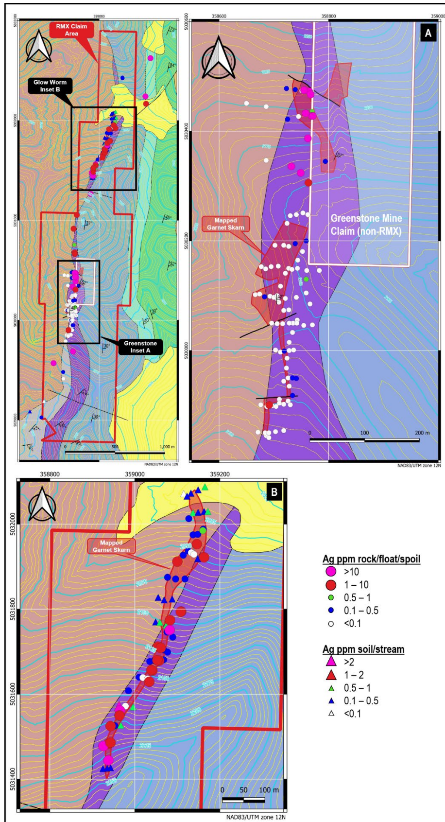
Figure 7: Silver (Ag) results for the Greenstone and Glow Worm prospects relative to topography and USGS surface geology after McDonald and Yakovlev (2019) 27 and mapped garnet skarn after Pattee (1960) 28 . For geology legend refer to Figure 3.
