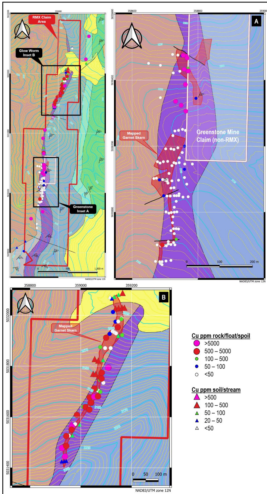
Figure 6: Copper (Cu) results for the Greenstone and Glow Worm prospects relative to topography and USGS surface geology after McDonald and Yakovlev (2019) 25 and mapped garnet skarn after Pattee (1960) 26 . For geology legend refer to Figure 3.
