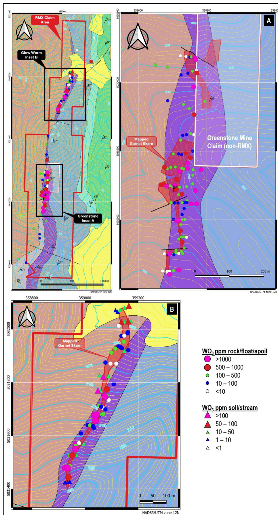
Figure 4: WO 3 results for the Greenstone and Glow Worm prospects relative to topography and USGS surface geology after McDonald and Yakovlev (2019) 16 and mapped garnet skarn after Pattee (1960) 17 . For geology legend refer to Figure 3.
