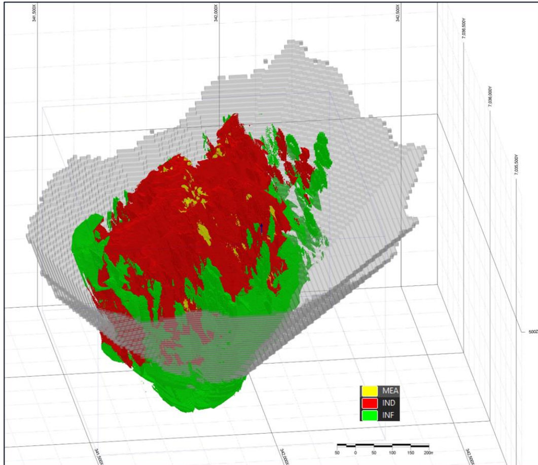
Figure 2: Isometric view of the Terner Gold Deposit block model looking north-west. Showing Measured (yellow), indicated (red) and Inferred (green) classified resources and US$3500/oz pit shell. Datum PSAD56 19S.
