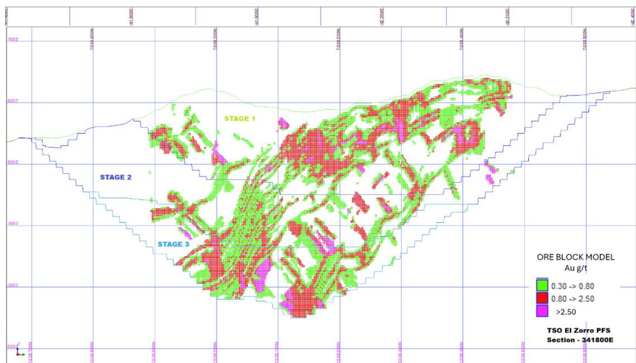
Figure 4: Ternera Deposit Ore Reserve Pit Section 7036200N (looking North)
