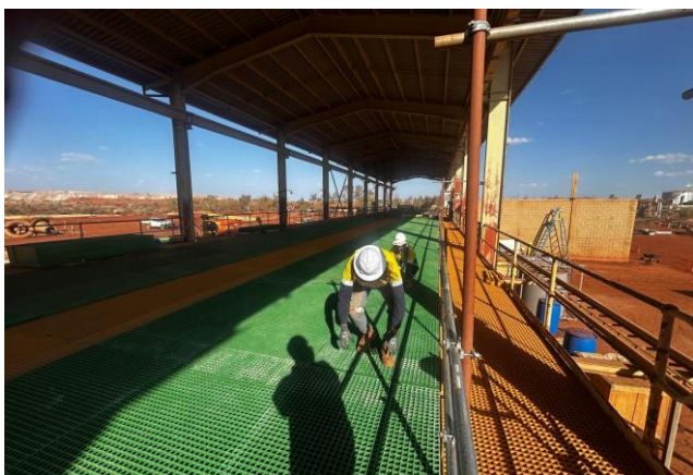
EW tank house flooring installed
