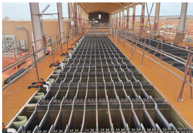
Cell top furniture and anodes installed
