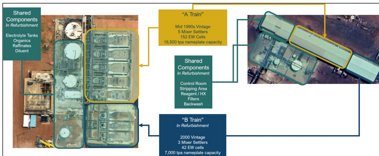
Nifty SXEW plant, process trains and shared components
