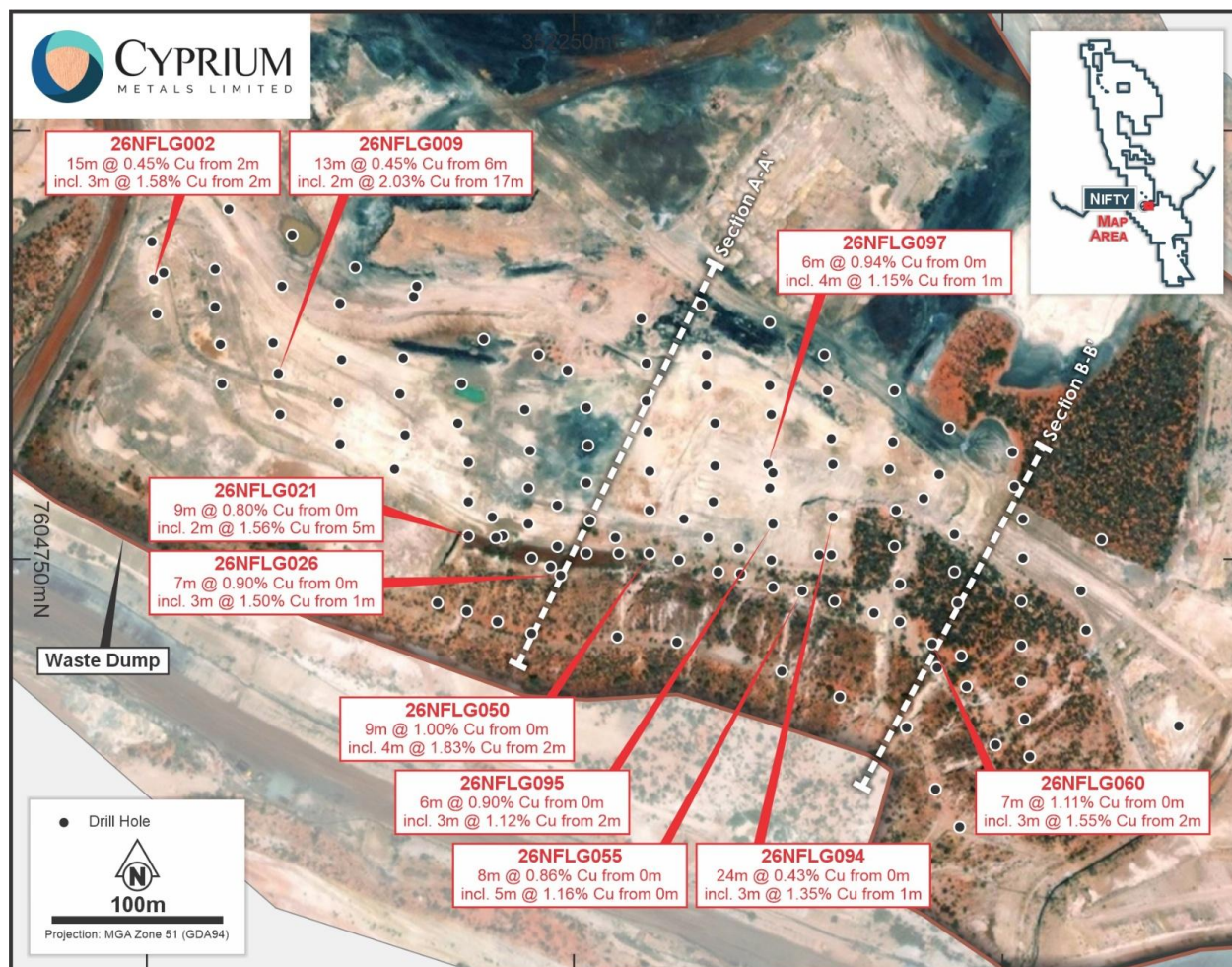
Primary mineralised zone within the Nifty waste dump with key intersections
