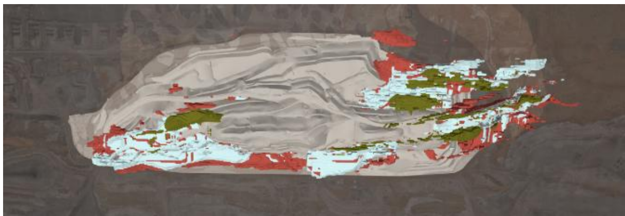
Oxide Resource location (looking up and north)
