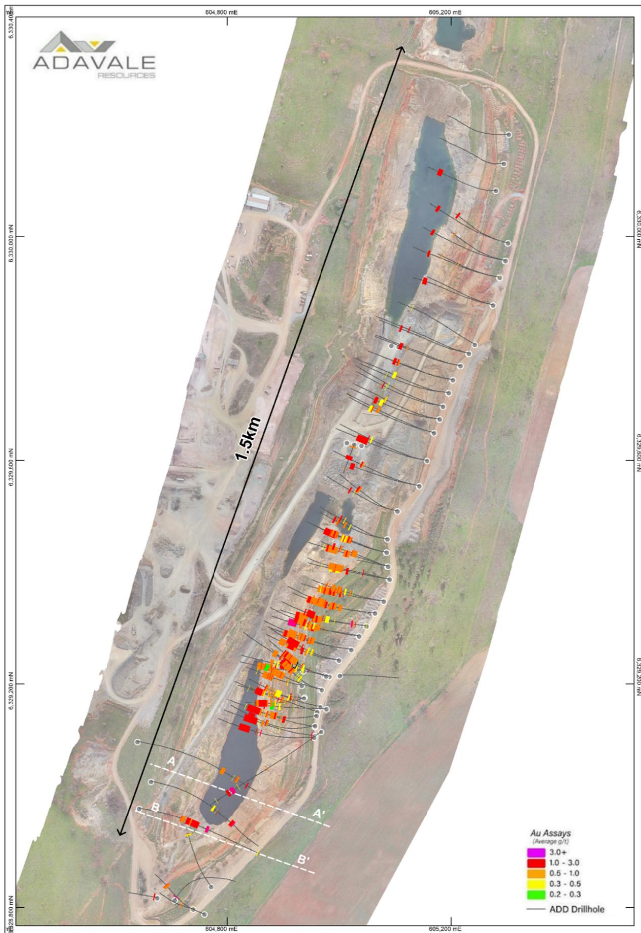
Figure 3: Plan view of the London-Victoria open pit displaying all Adavale drillholes
