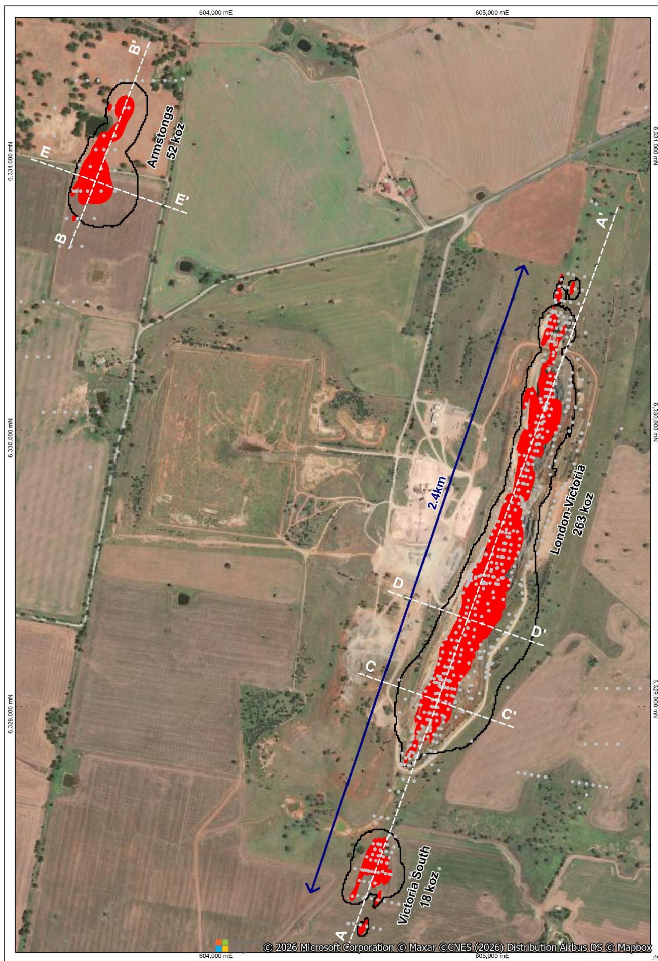
Figure 2: Plan view of mineralisation wireframes, drillhole collars and the USD$4,200/oz pit optimisation shell
