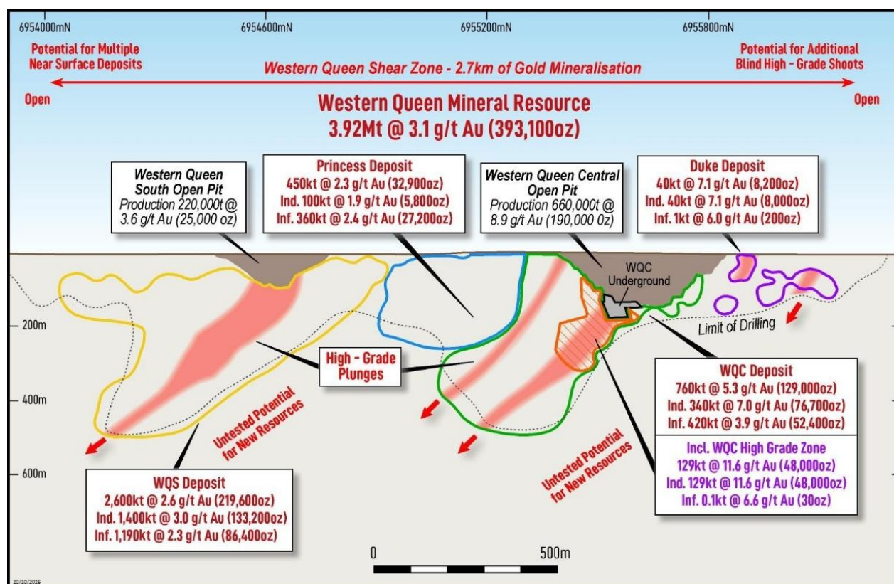
Figure 3 – Western Queen Gold Deposit Longitudinal Section – Highlighting Previous Production, Resources and Potential New Resource Areas
